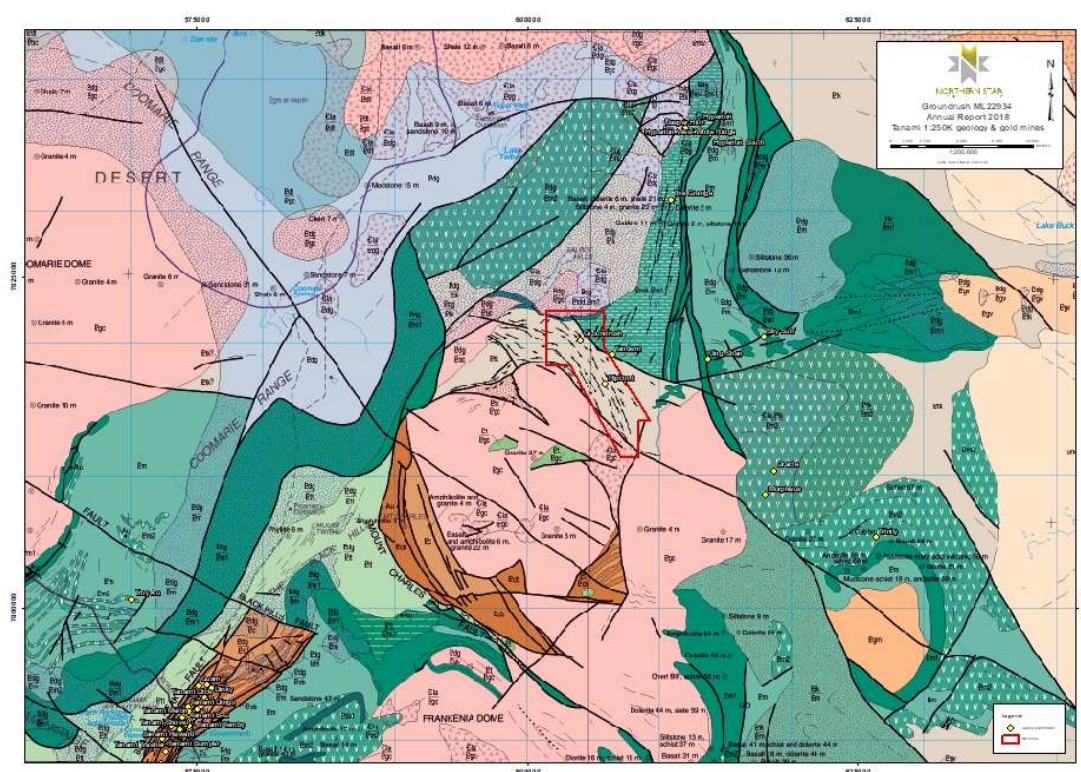
Figure 2: Tanami 1:250,000 NTGS regional interpreted bedrock geology with gold occurrences
