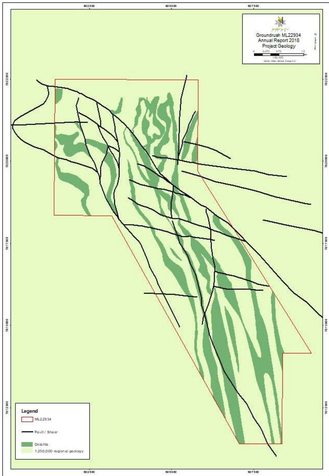
Figure 3: 1:50,000 project geology
