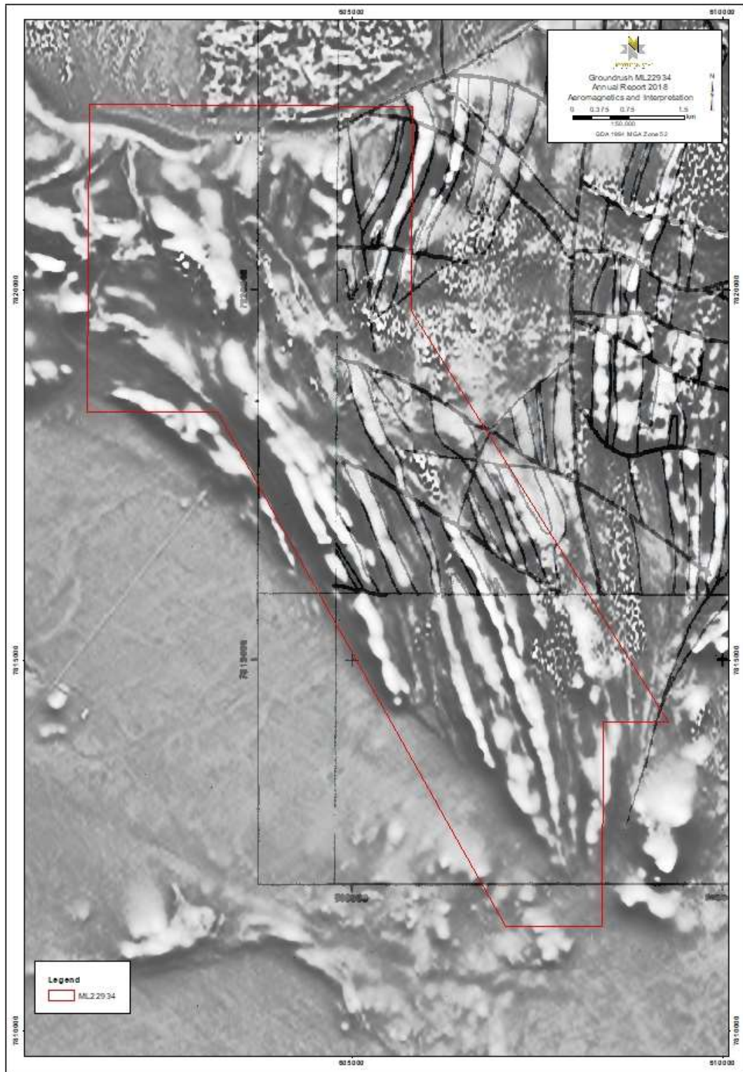
Figure 5: TMI with first vertical derivative filter and 1:50,000 geological interpretation
