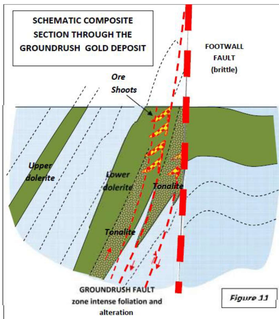
Figure 4: Schematic Composite Section after Marjoribanks (2011)
