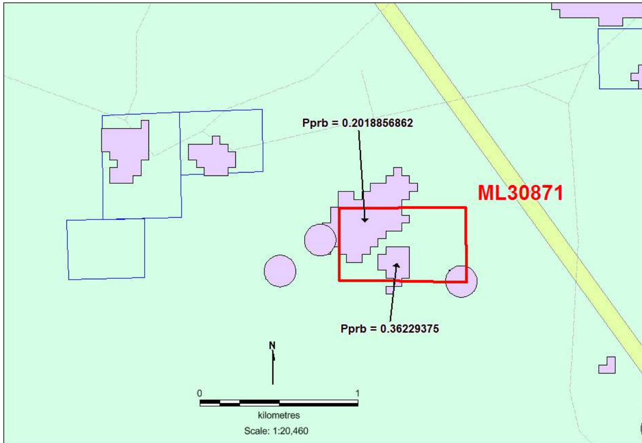
Figure 4: ML 30871 vs. Kenex generated targets (magenta polygons)
