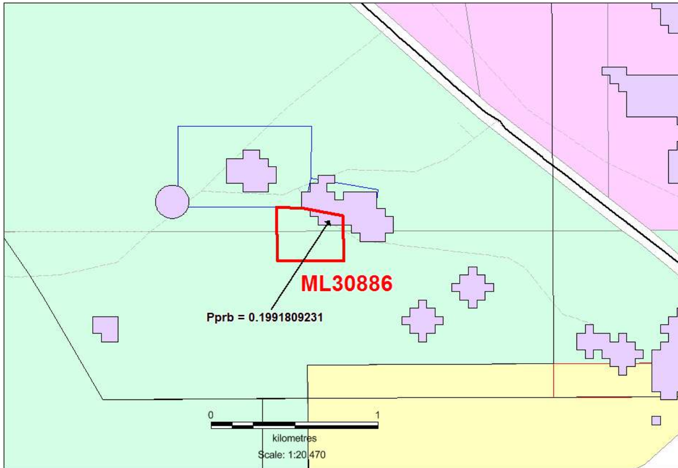
Figure 4: ML 30886 vs. Kenex generated targets (magenta polygons)
