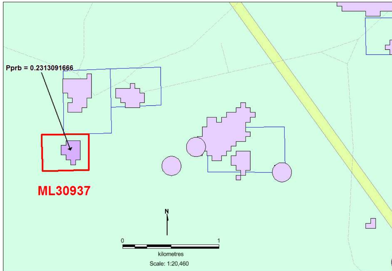
Figure 4: ML 30937 vs. Kenex generated targets (magenta polygons)
