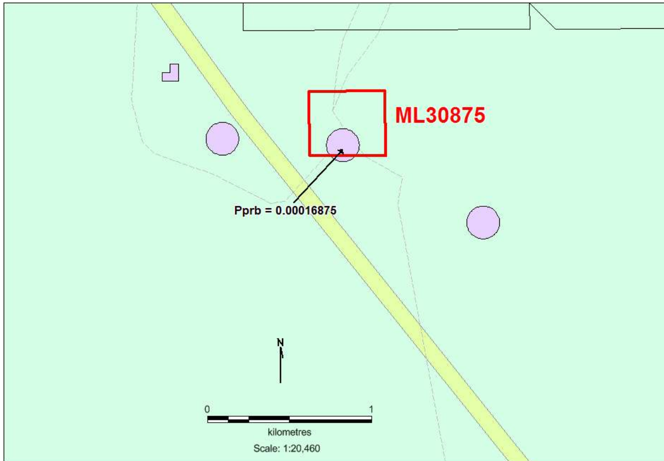
Figure 4: ML 30875 vs. Kenex generated targets (magenta polygons)
