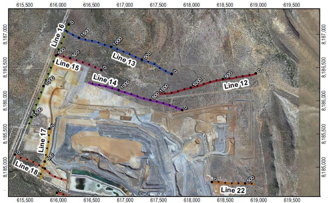
Figure 3: ERI lines completed on MLN1124. From Anderson, 2016
