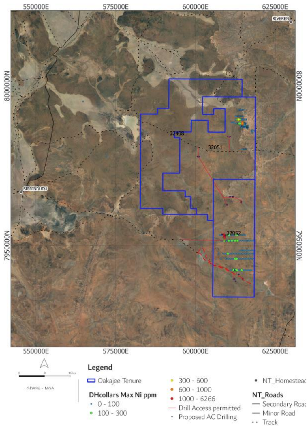
Figure 6 Birrindudu Drilling coloured by Max Ni ppm with proposed Aircore drilling and permitted Access.
