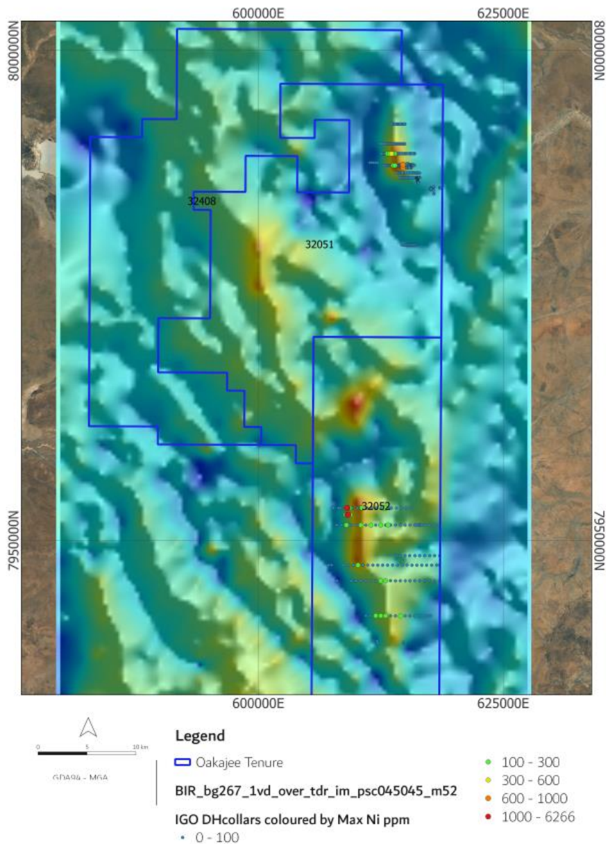
Figure 4 Birrindudu Drilling Max Ni ppm
