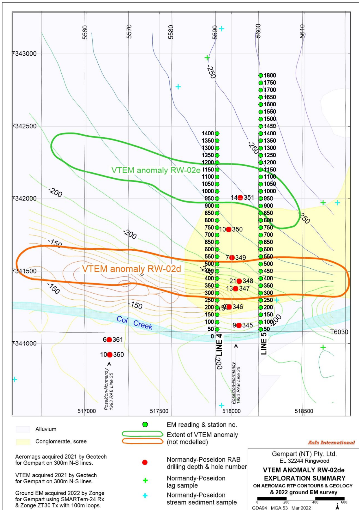
Figure 20. VTEM anomaly RW-02de exploration summary.
