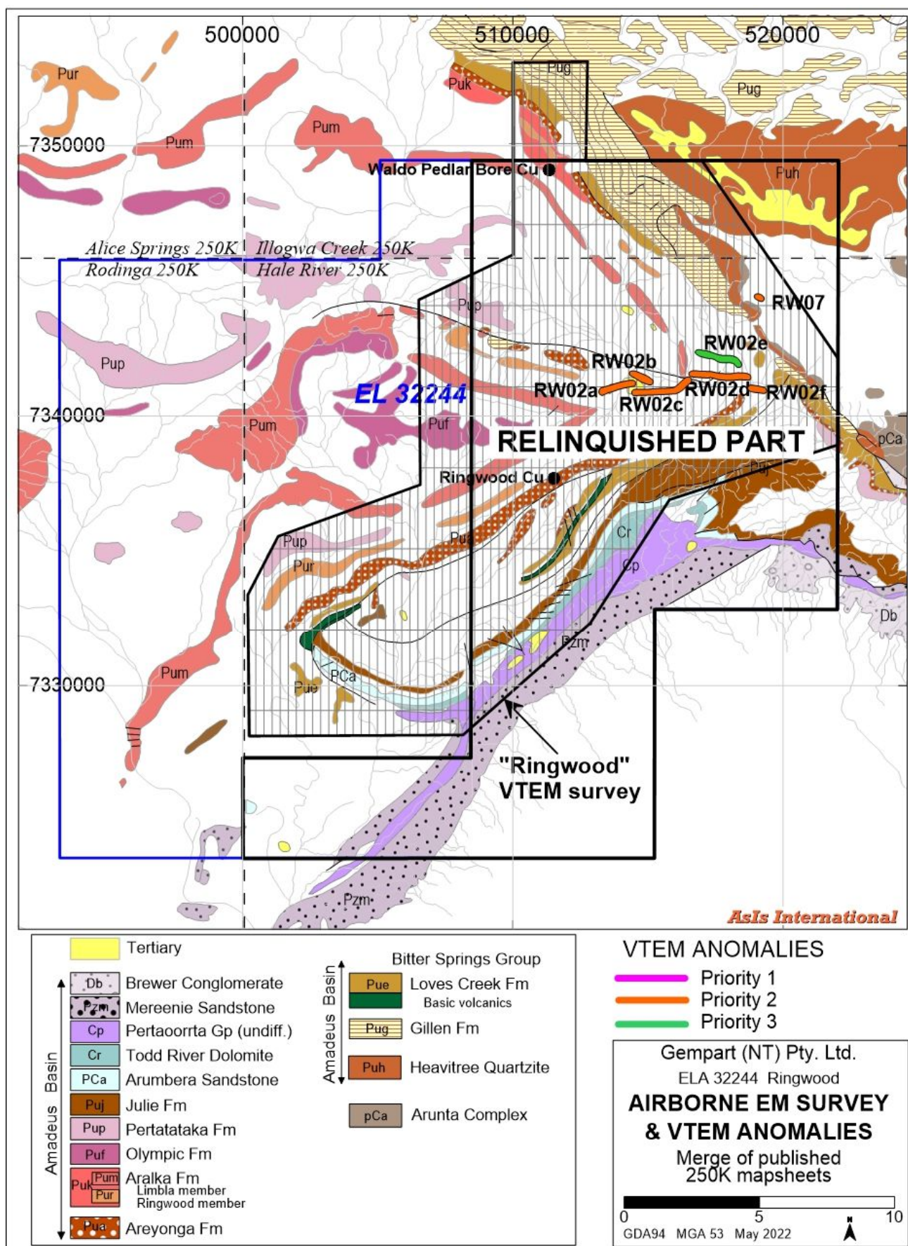
Figure 17. Location of Ringwood VTEM survey and anomalies on geology.
