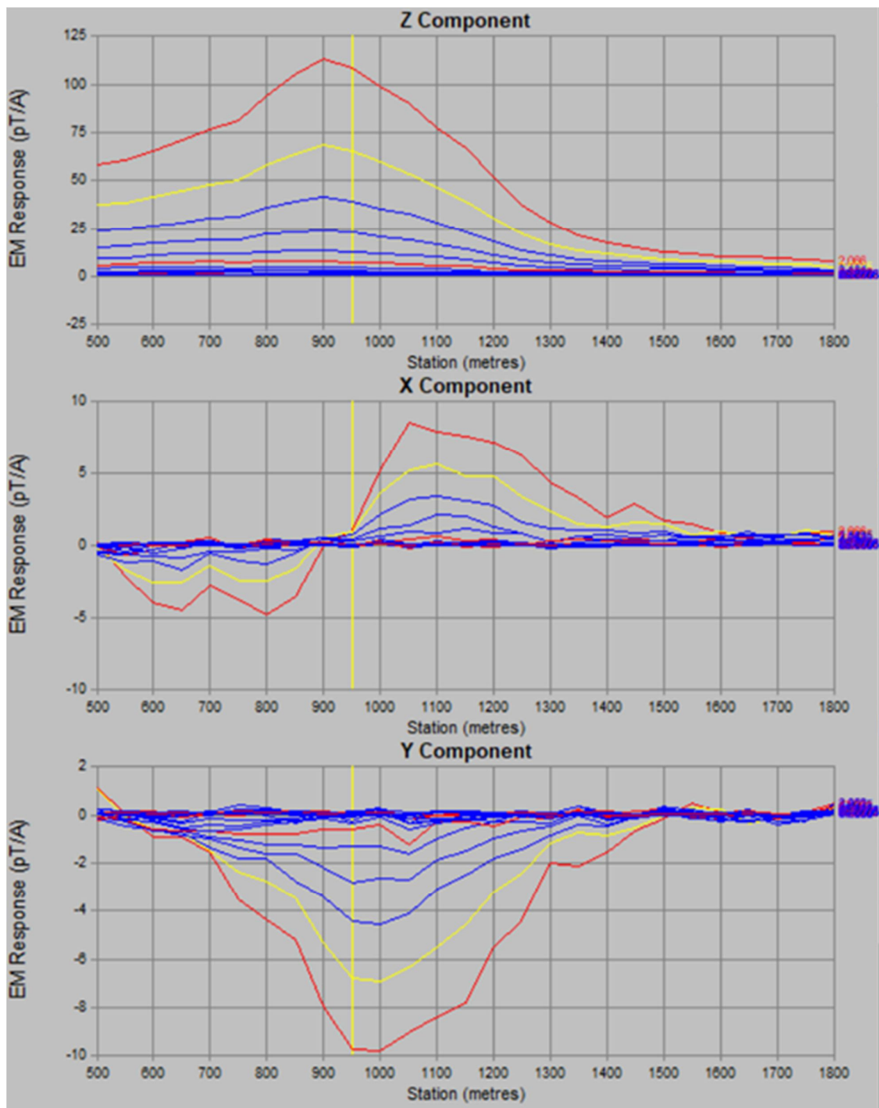
Figure 24. VTEM anomaly RW-02de Line 5 ground EM profiles (preliminary).
