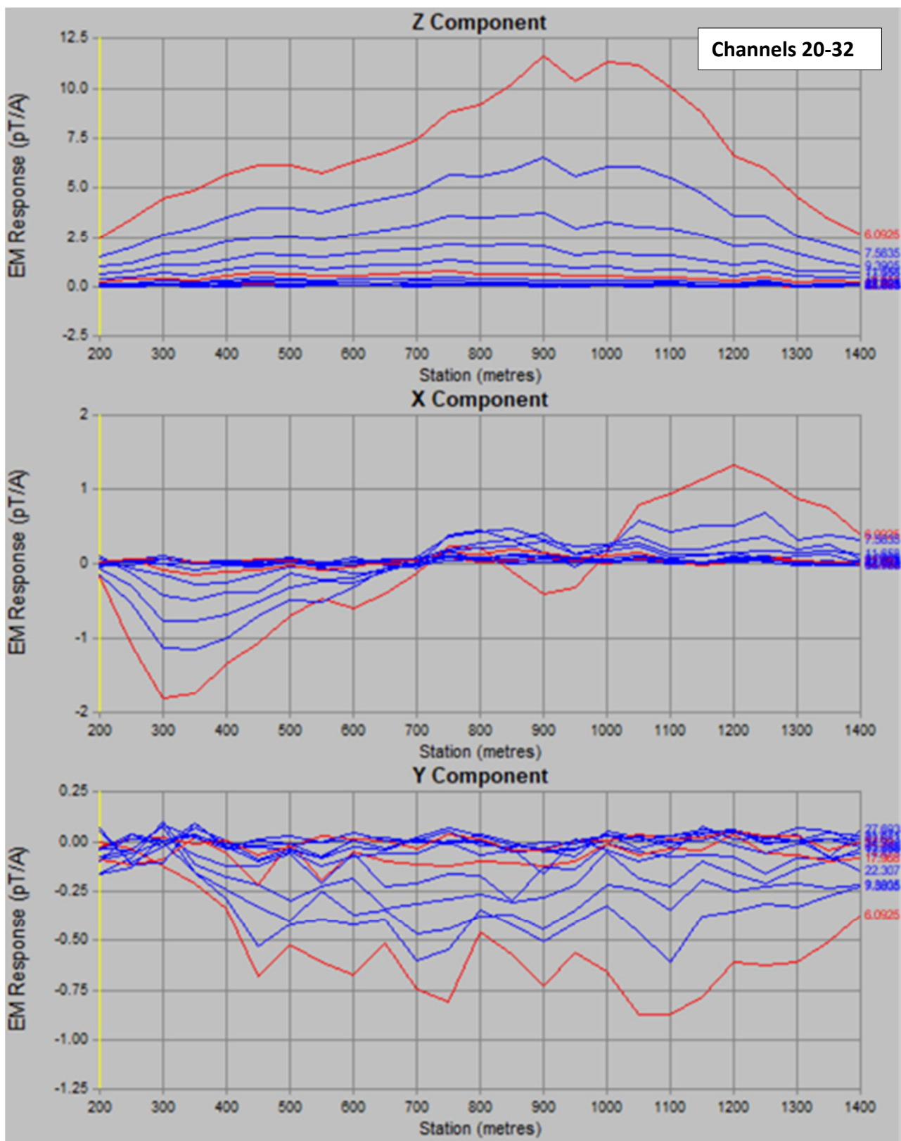
Figure 23. VTEM anomaly RW-02de Line 4 ground EM profiles (preliminary).
