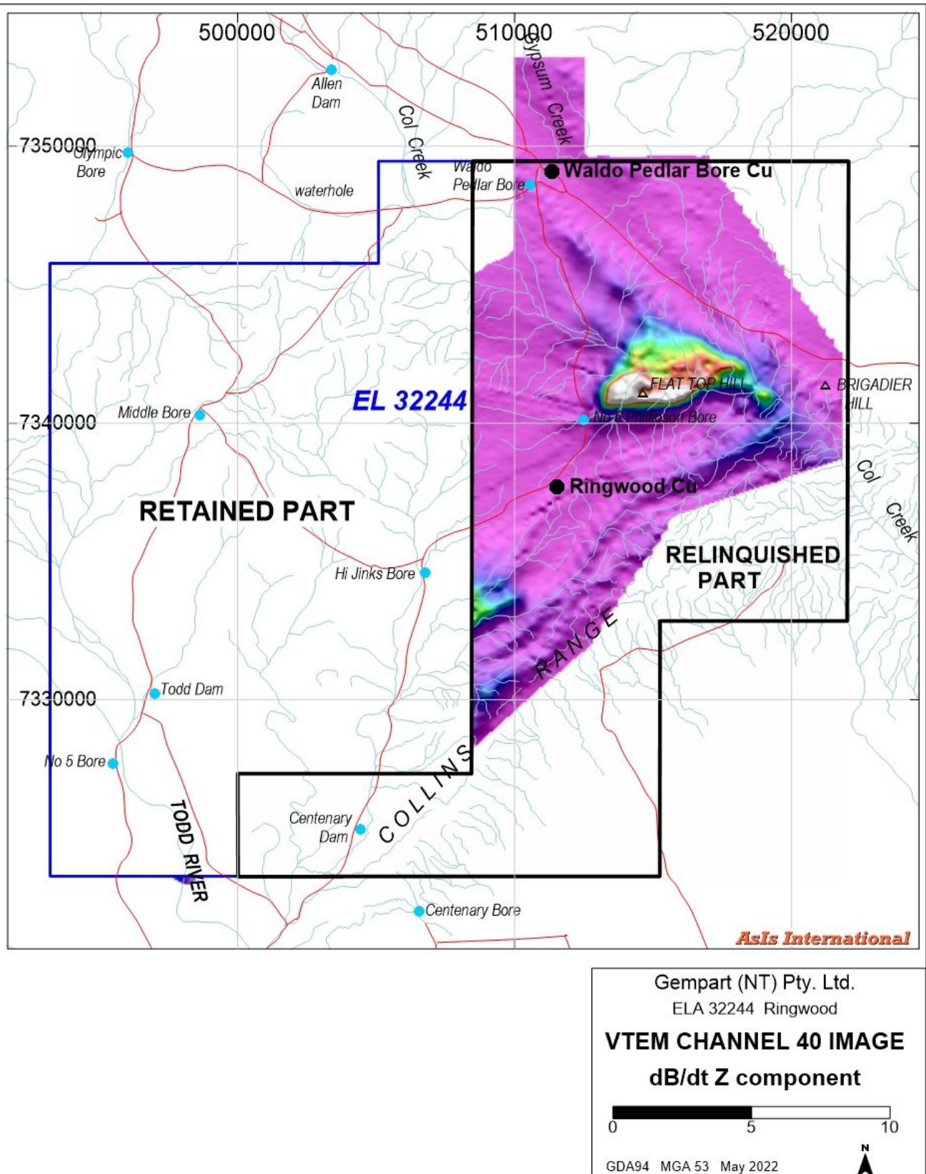
Figure 18. Ringwood VTEM image dB/dt Ch40Z.
