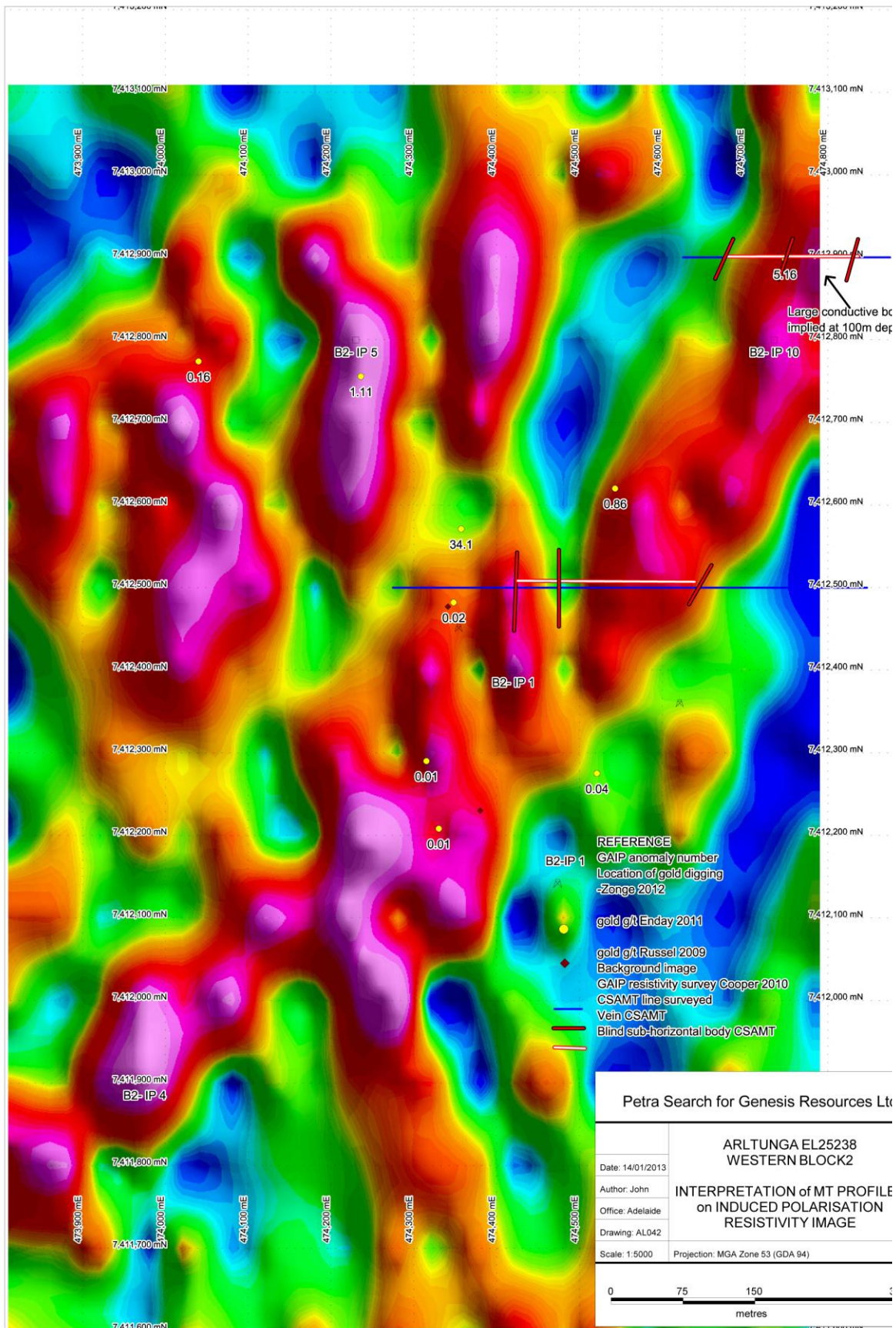
Figure 8 Location of western CSAMT profiles on GAIP resistivity image
