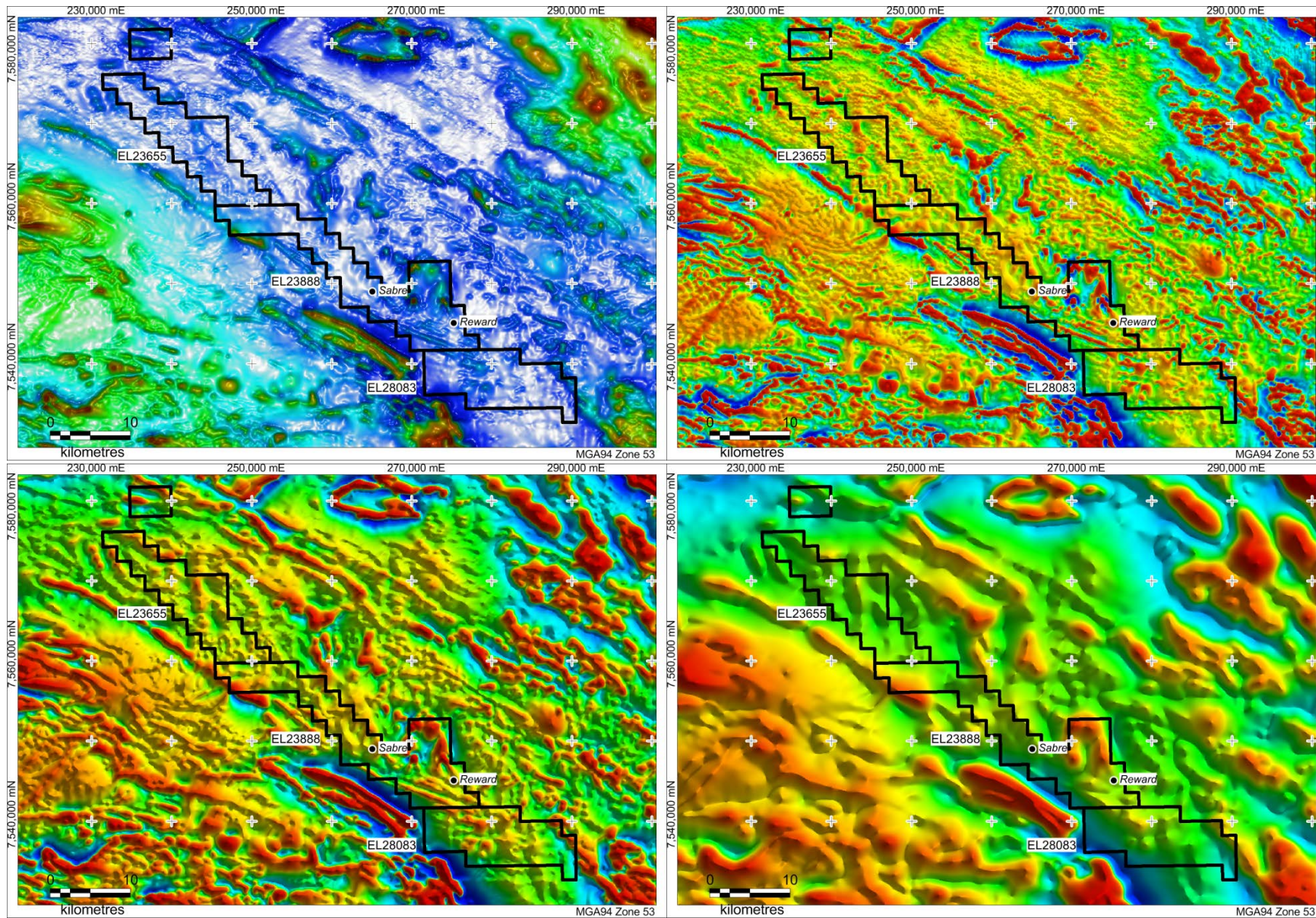
Figure 2 – Regional dRTP images for Reynolds Range. From top left dRTP vertical illumination then clockwise shallow, deep and intermediate residuals.
