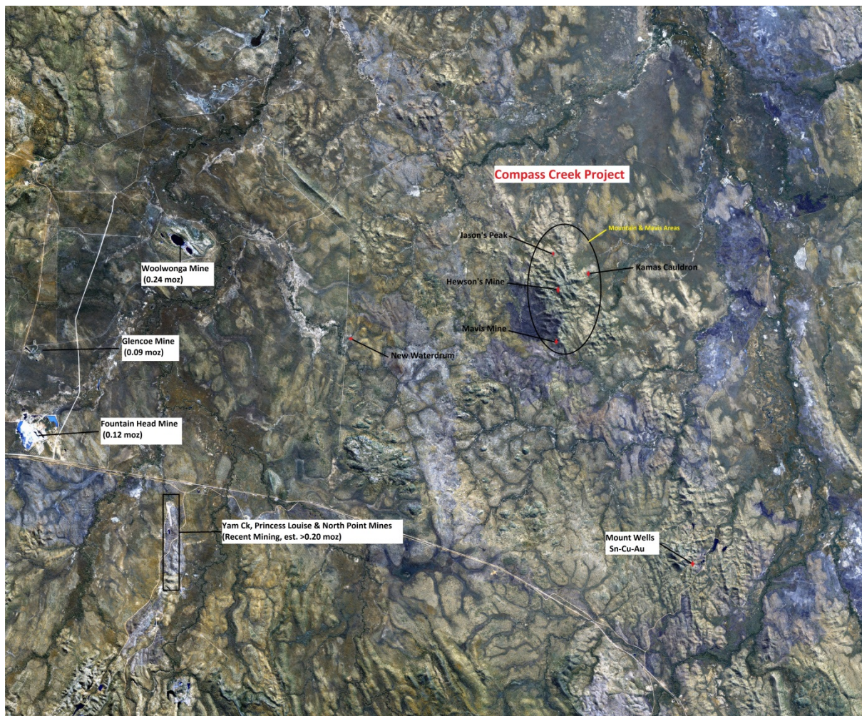
Figure 1: Satellite (Spot) Imagery showing the elevated “Mountain & Mavis Area” in the Compass Creek Project, plus the location of nearby gold & tin mines.
