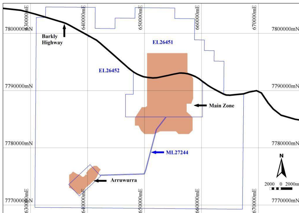
Figure 2: Resource areas and tenement boundaries
