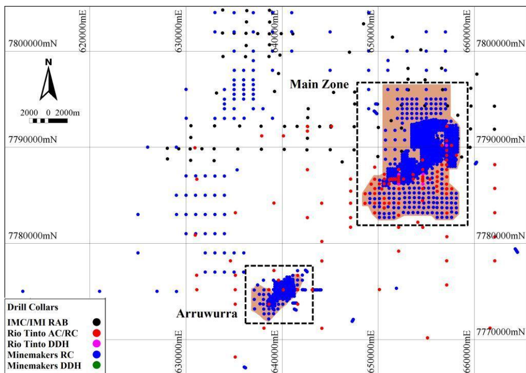
Figure 8: Model extents and drill hole collars
