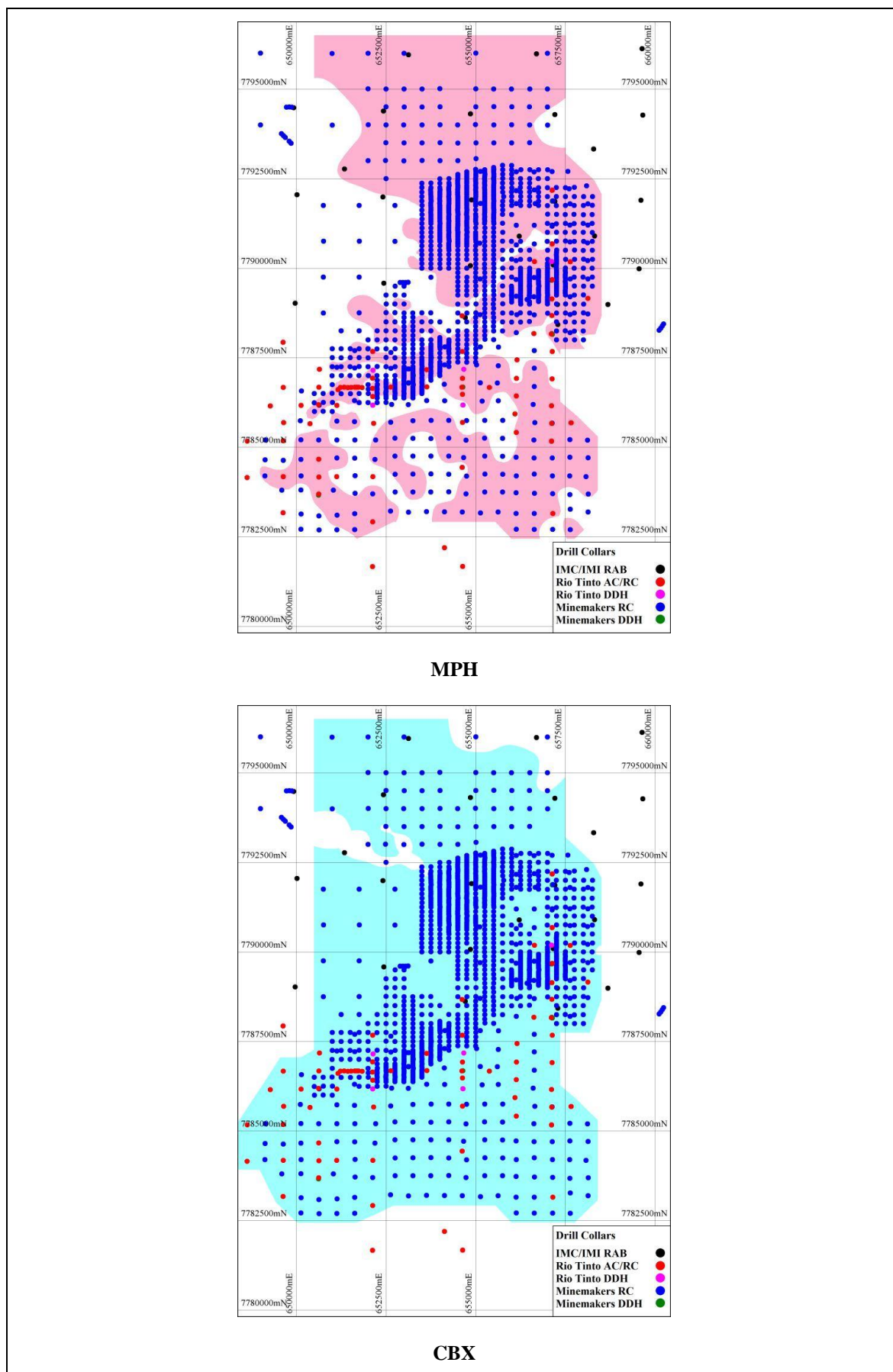
Figure 7: Main Zone major mineralized domains relative to drill hole collars
