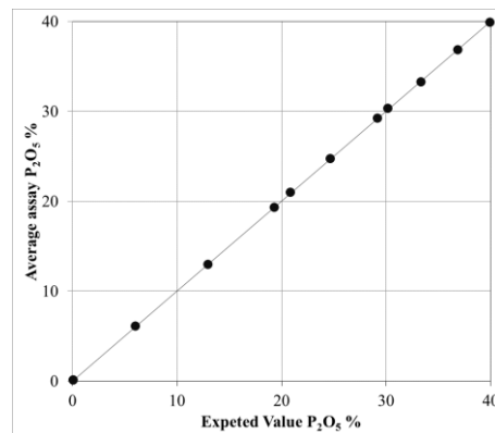
Figure 11: Reference standards \text{P}_2\text{O}_5 assays versus expected values
