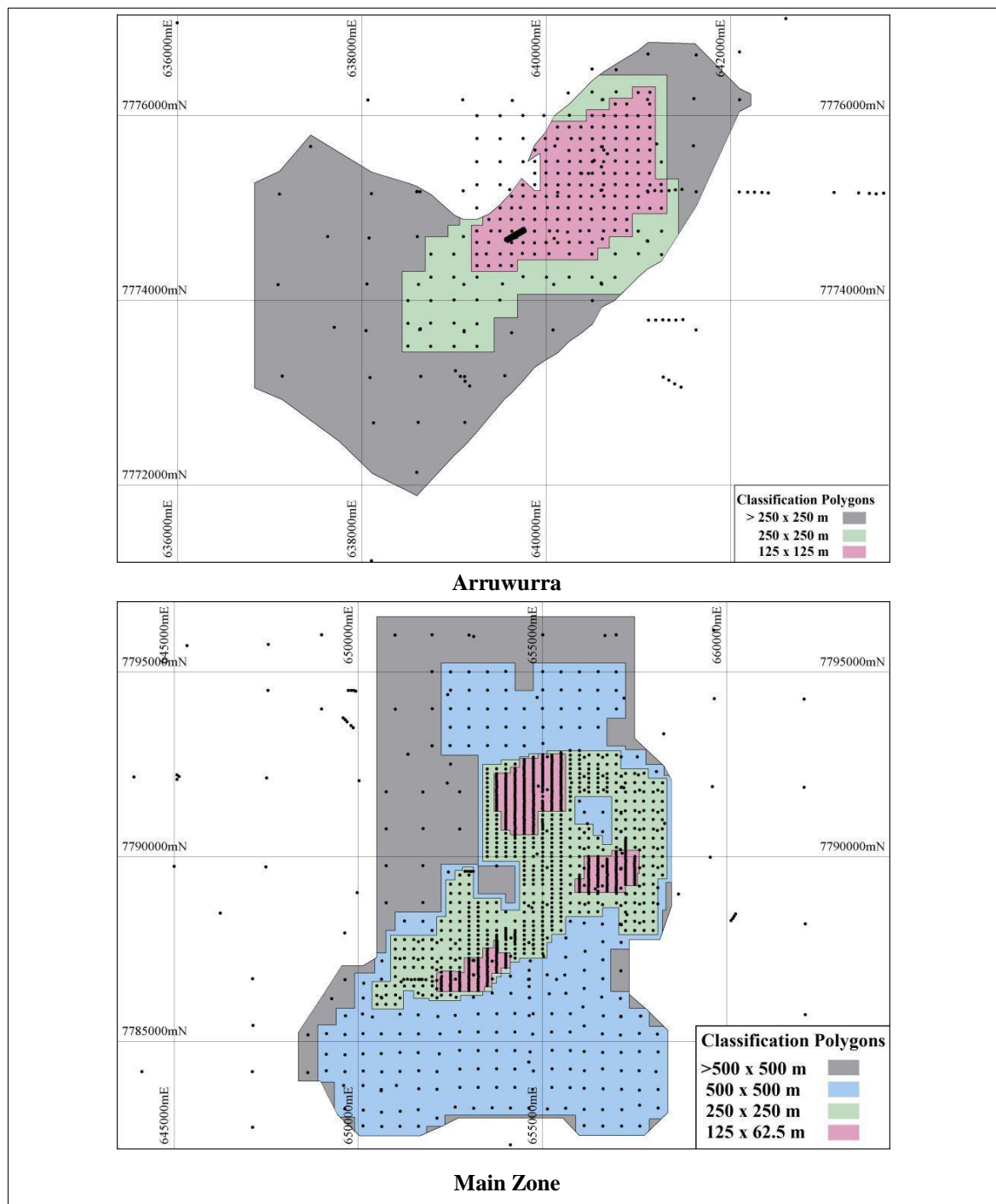
Figure 12: Resource classification polygons
