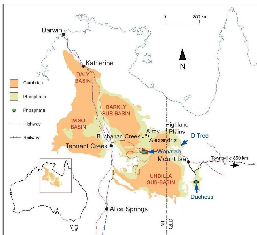
Figure 3: Regional geological setting and phosphate deposits
