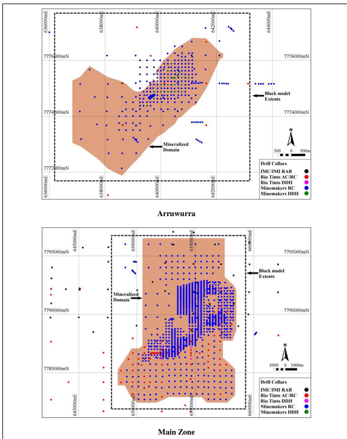
Figure 4: Combined mineralized domains, drill hole collars and model limits
