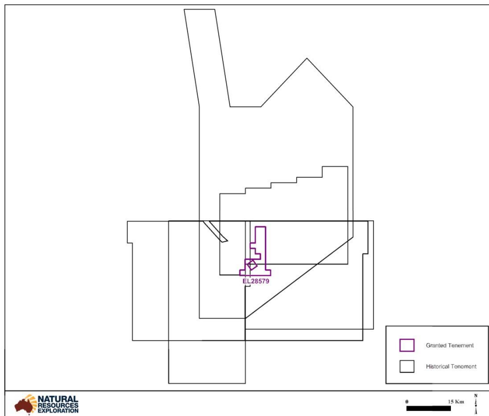
Figure 9. Historic tenements over EL28579
