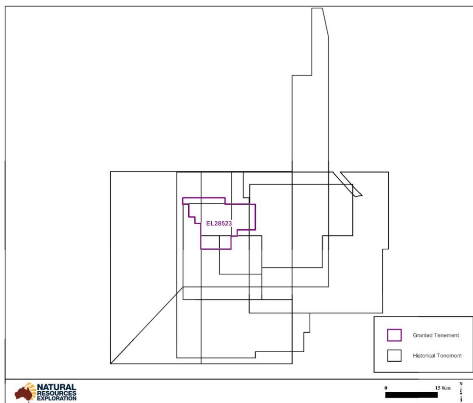
Figure 8. Historic tenements over EL28523
