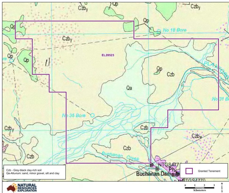
Figure 7. Permit Geology Map
