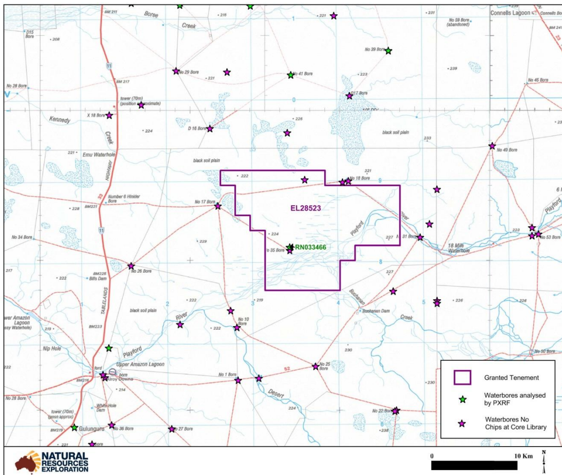
Figure 9. Water Bore Location Map
