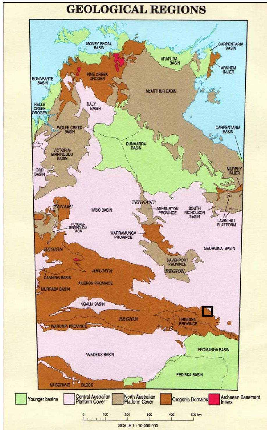
Figure 2. Geological Regions of the Northern Territory (image from Ahmad and Scrimgeour, 2004) showing the approximate area of interest for Jervois project area and EL 26231.
