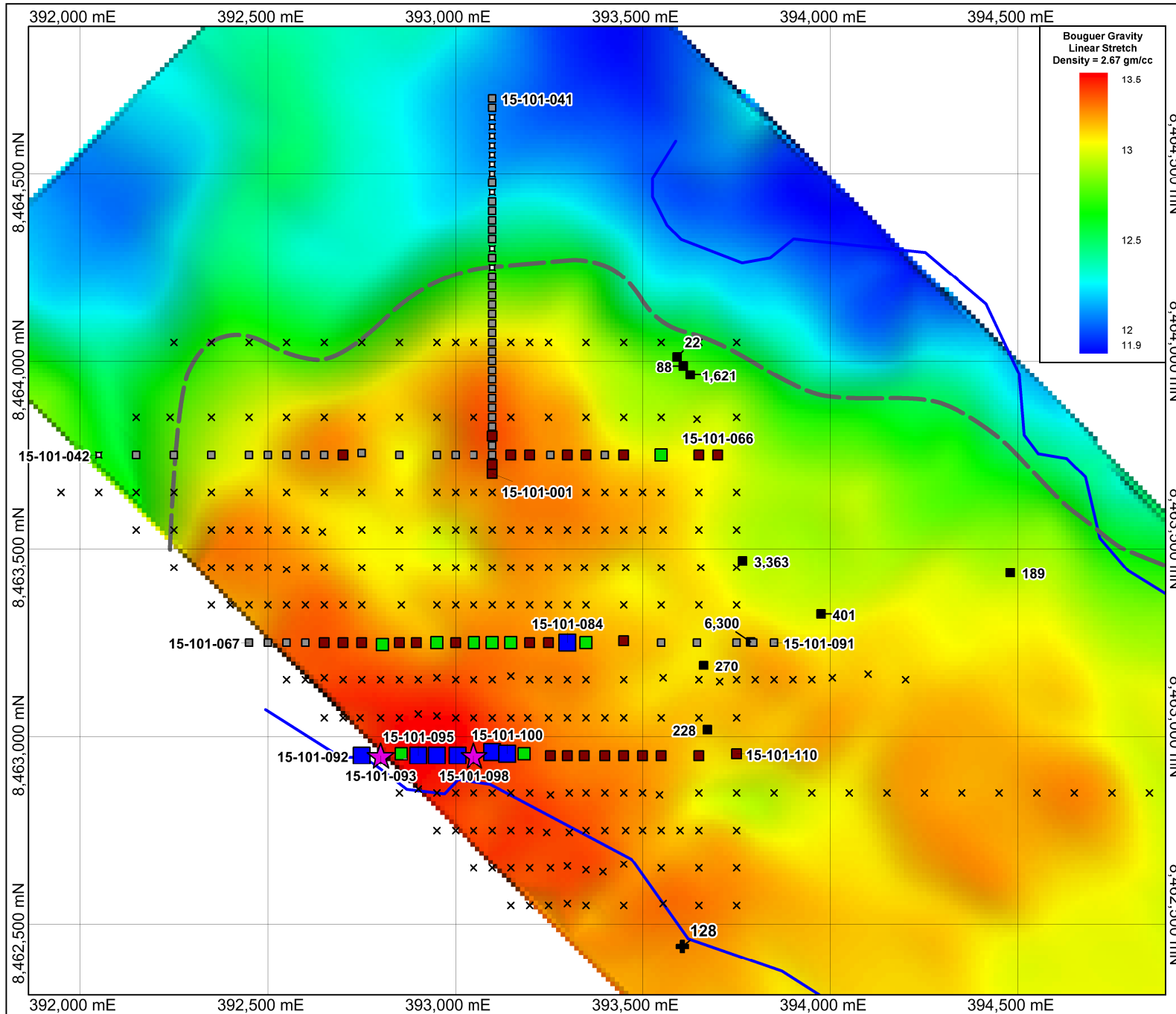
BACKGROUND: Bouguer Gravity - Daishsat Survey Data (2013)
