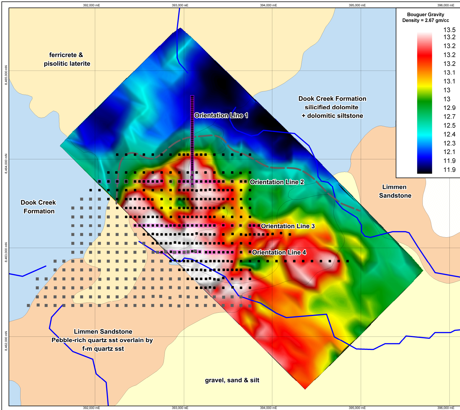
BACKGROUND: Bouguer Gravity - Daishsat Survey Data (2013) overlying Mt Marumba (SD53-06) geology
