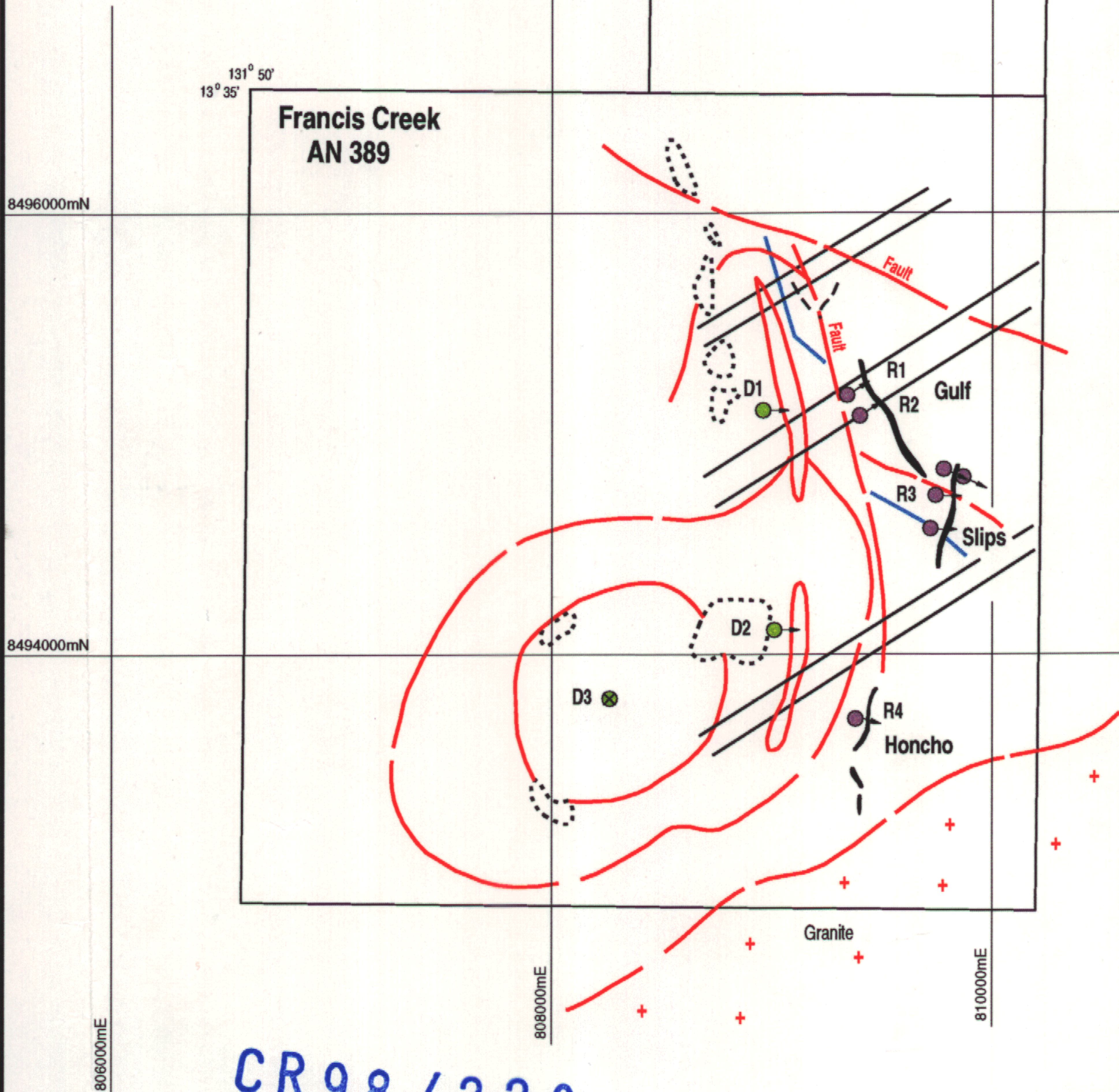
Francis Creek Project Summary Geological Features Figure 26
