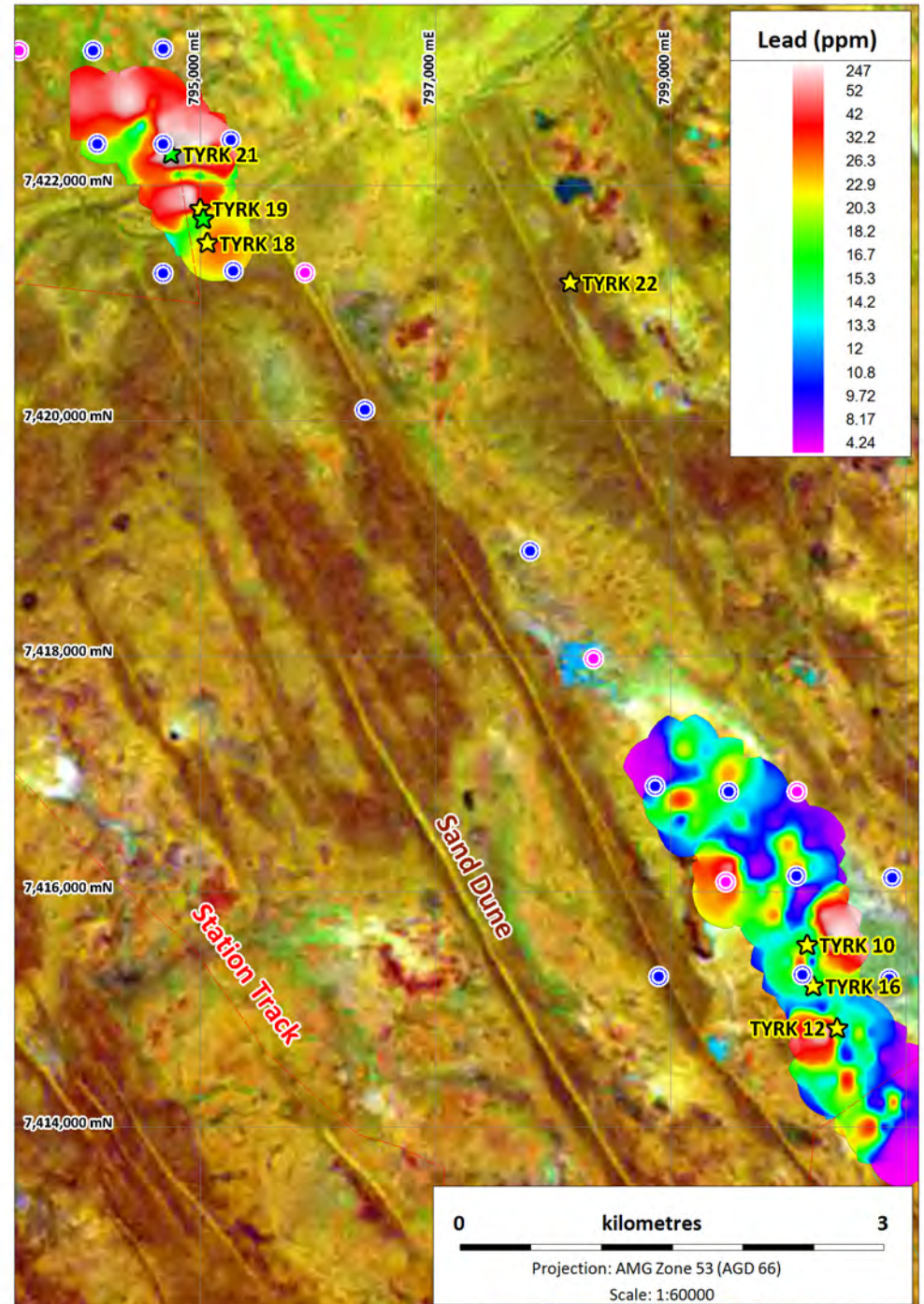
Elstone Prospect Lag Sampling Results and Grab Samples (yellow) on Landsat Showing Proposed Drill Holes (priority blue and secondary pink)
