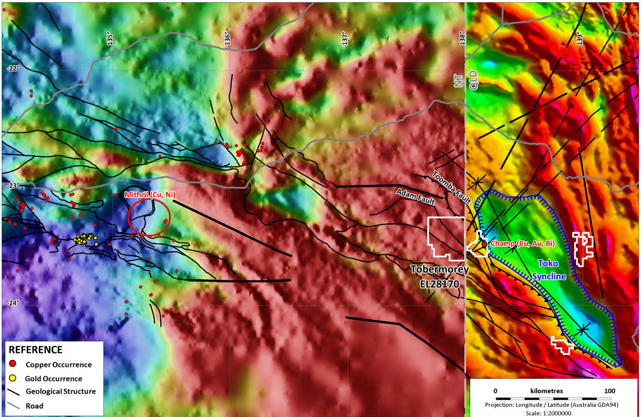
Diamantina Project NT/QLD Government Gravity Images Showing Regional Structures and Mineralisation
