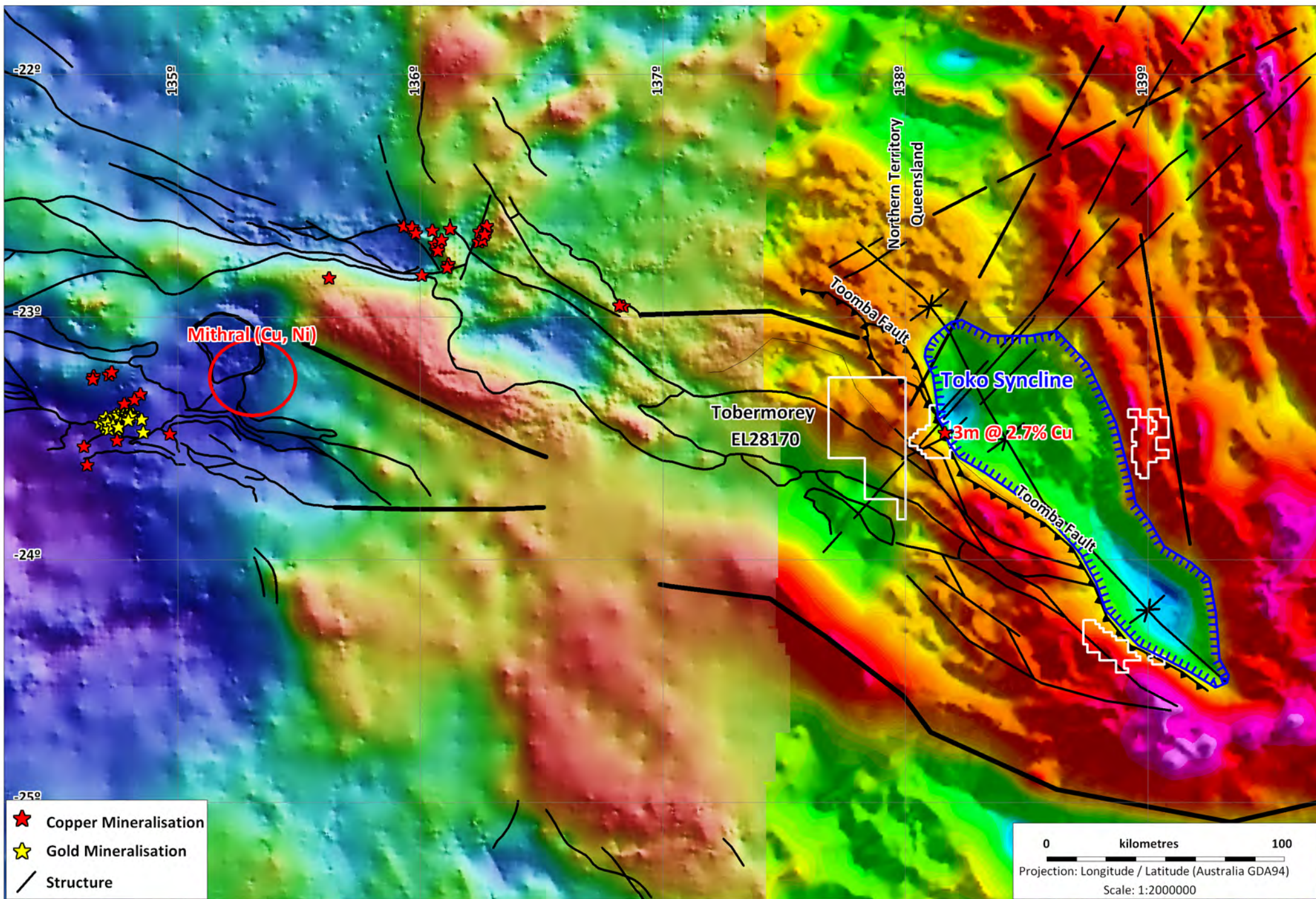
Tobermorey EL28170 - Government Gravity Image with Structures and Mineralisation
