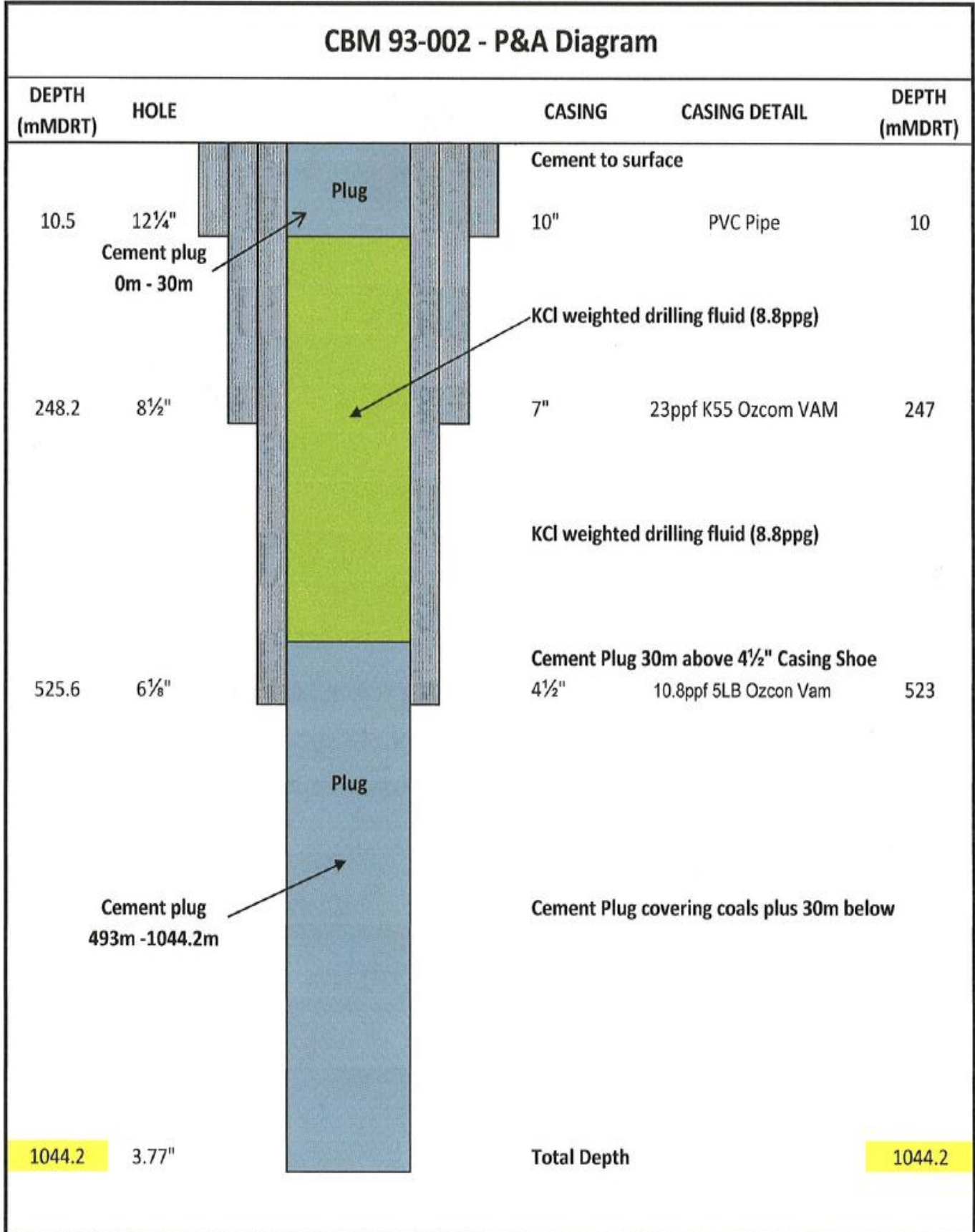
Figure 3: CBM 93-002 P&A diagram.
