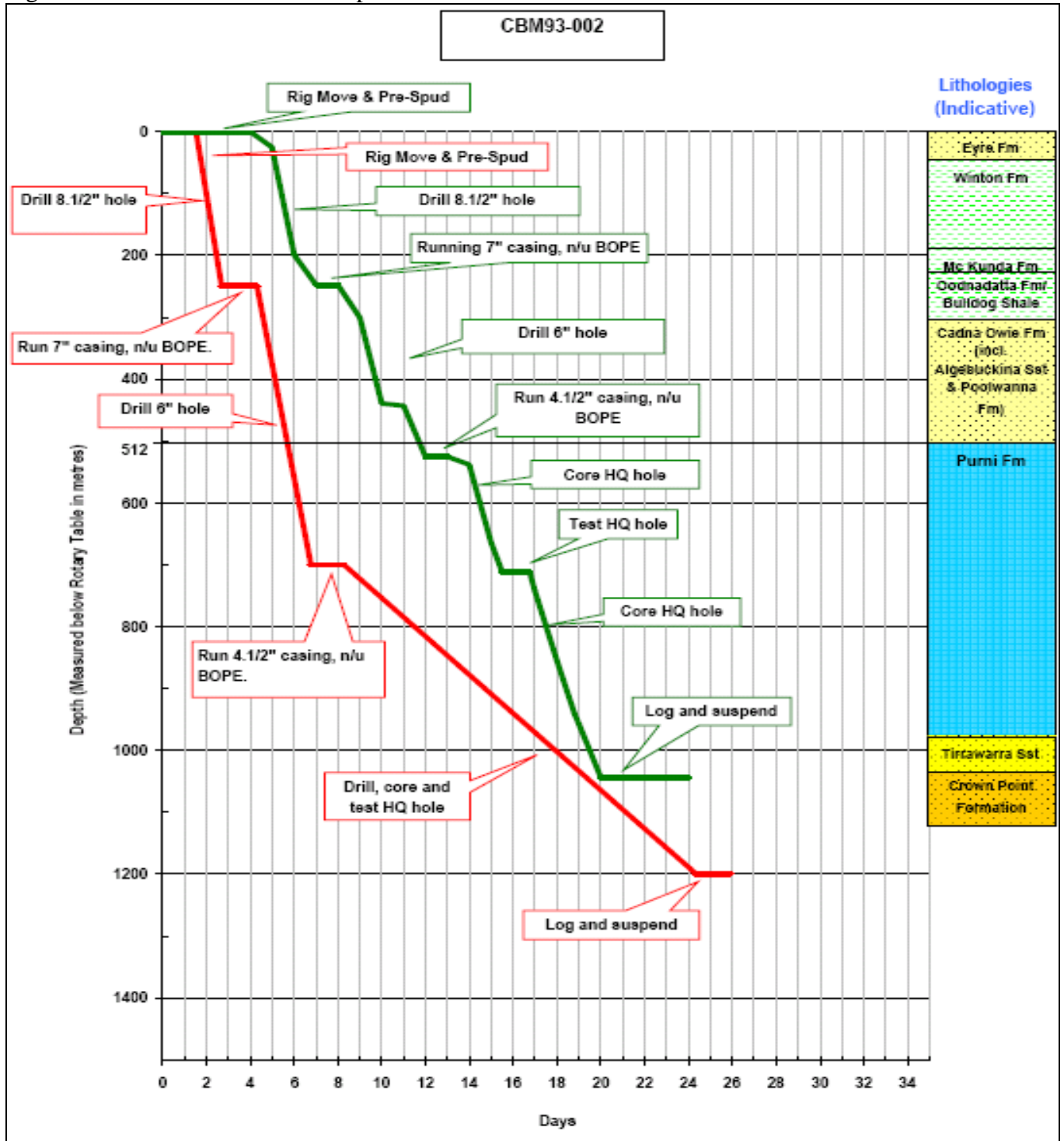
Figure 2: CBM 93-002 Time vs Depth chart.
