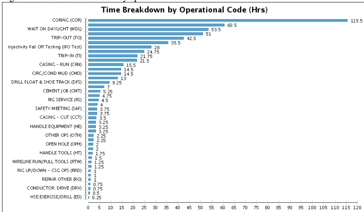
Figure 4: Lost time breakdown by operational code.
