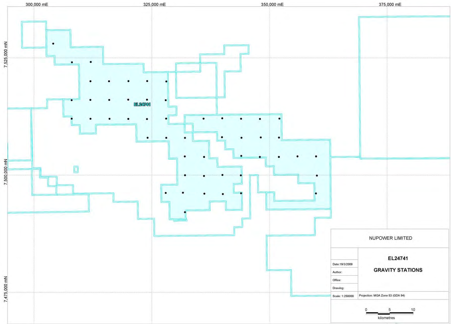
Central Arunta Gravity Survey (CAGS) Stations
