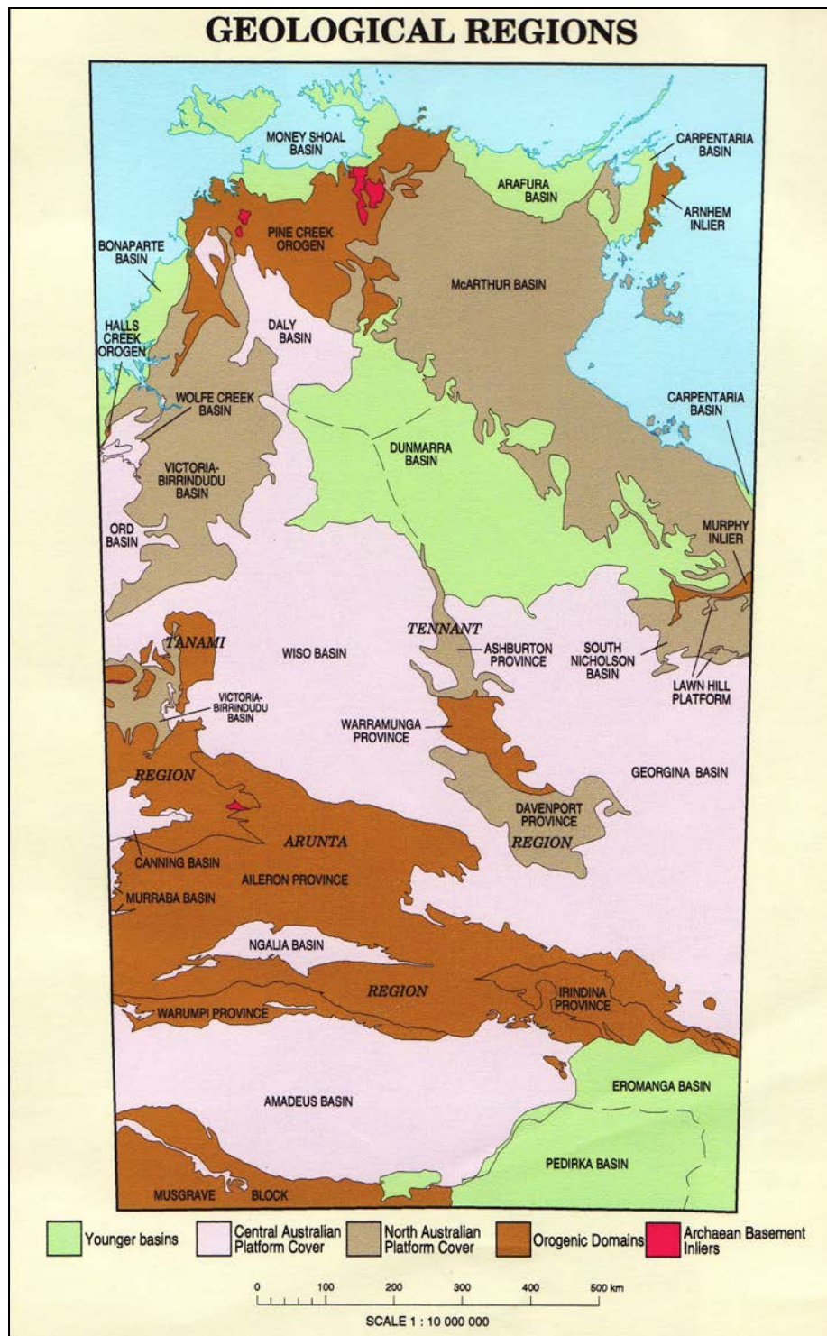
Figure 1. Geological Regions of the Northern Territory (image from Ahmad and Scrimgeour, 2004).
