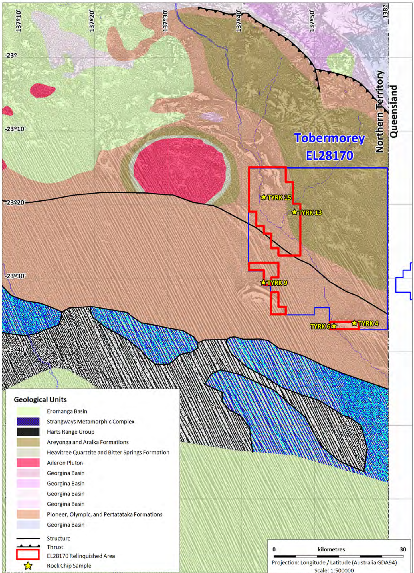
Tobermorey EL28170 - Government Geology Plan
