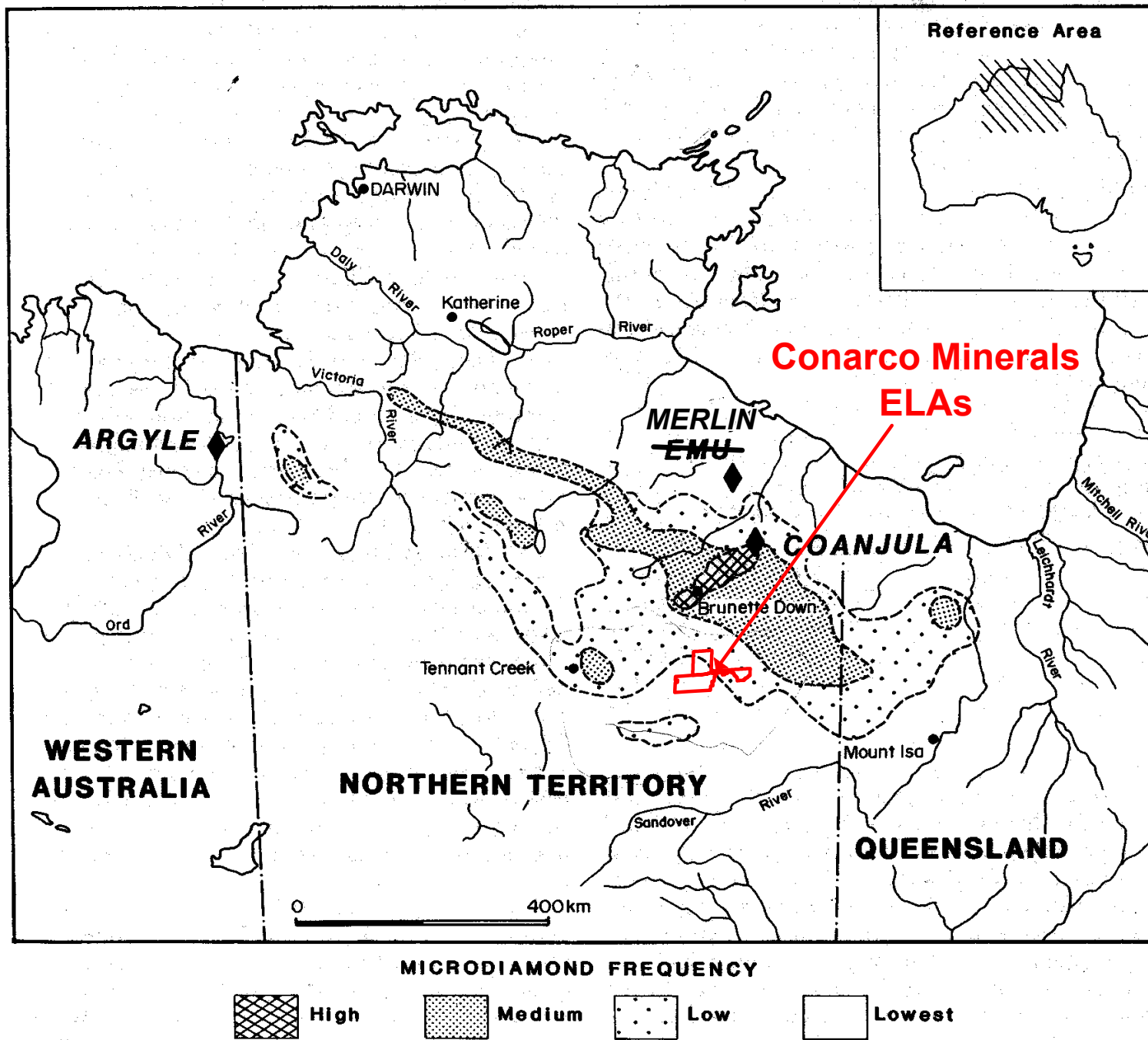
FIG. 11—Distribution of microdiamonds and kimberlitic pipes in the Northern Territory and adjacent portion of Queensland.
