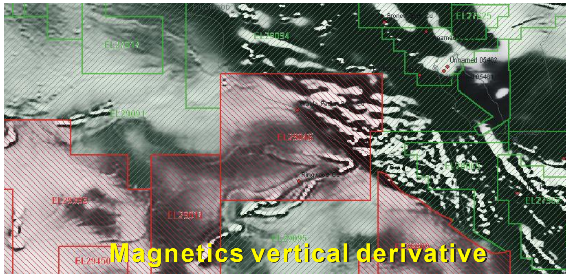
Fig. 3 Aero-magnetic Images at EL29046
