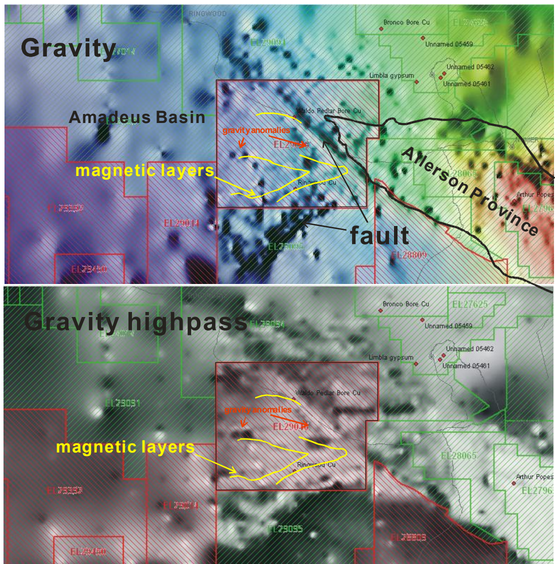
Fig. 4 Aero-gravity Images at EL29046
