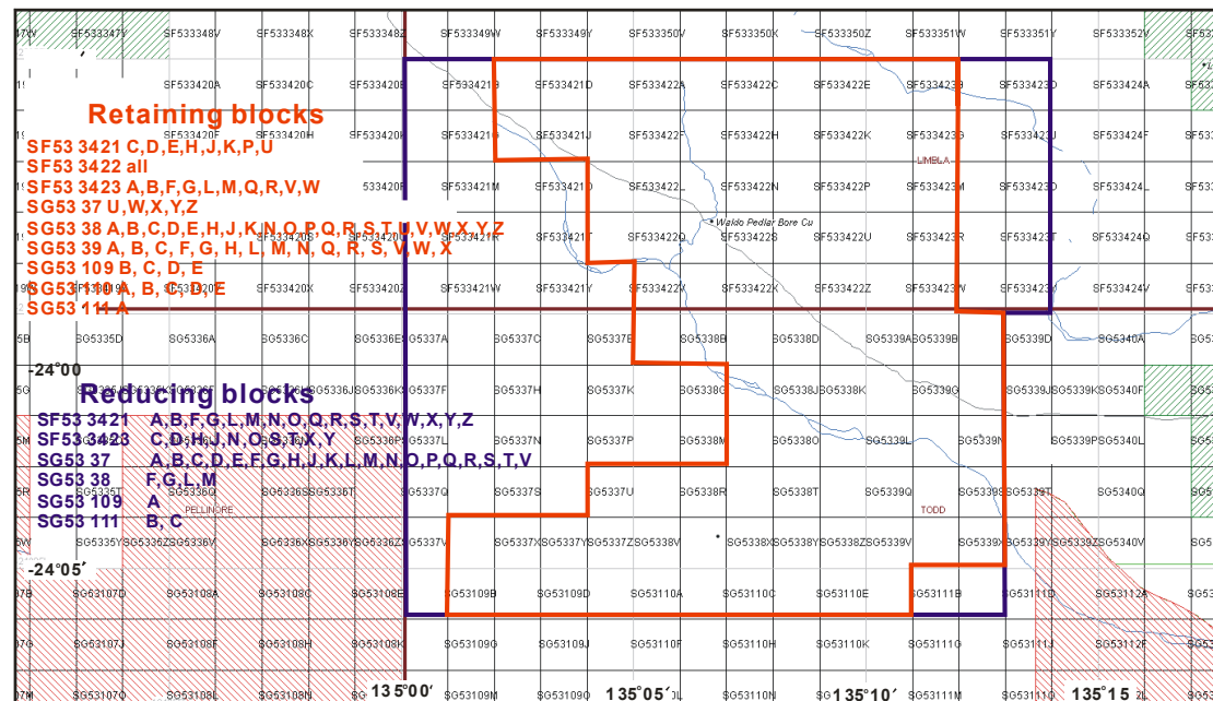
Fig. 1 Showing retaining and reducing blocks in EL29046.
