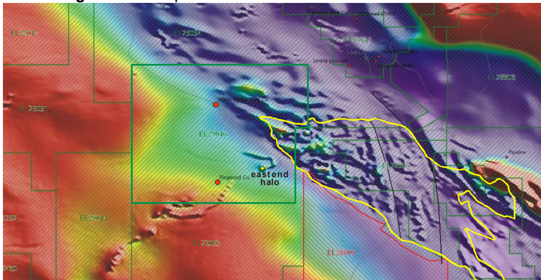
Fig. 2 Landscape of EL29046 and two mineral occurrences.
