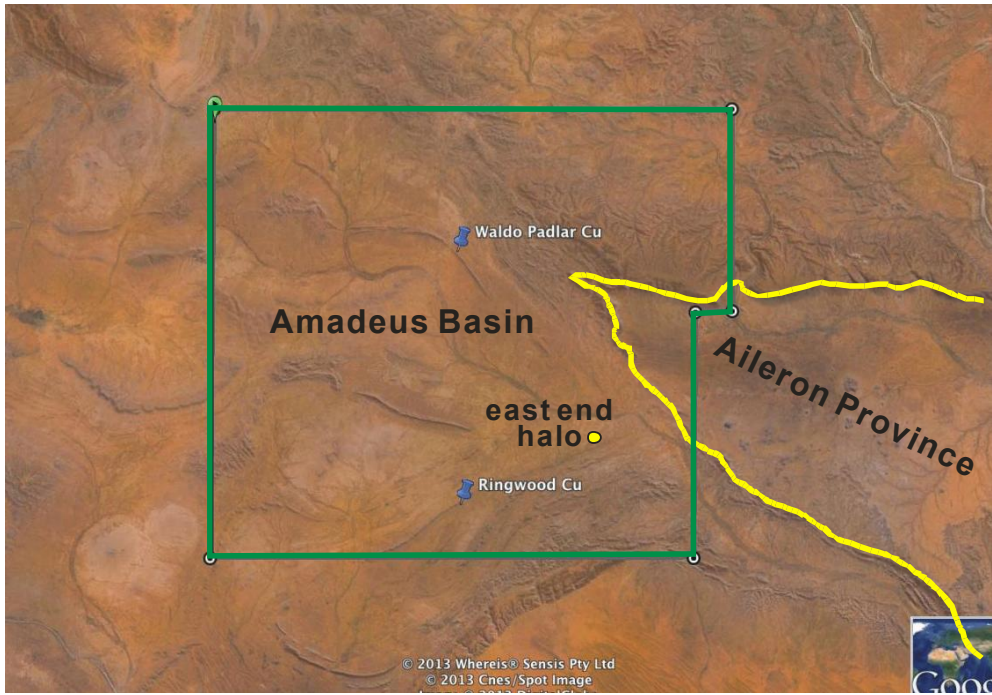
Fig. 2 Landscape of EL29046 and two mineral occurrences.
