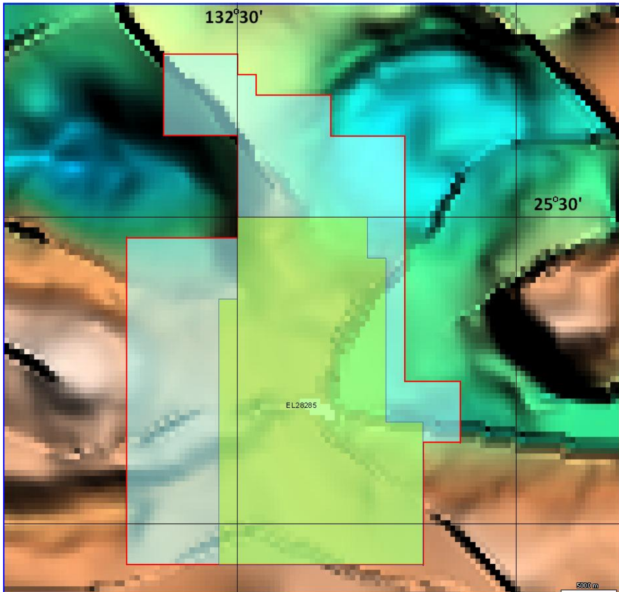
Figure 3: EL 28285 Seebase image showing potential structures within relinquished areas (blue)
