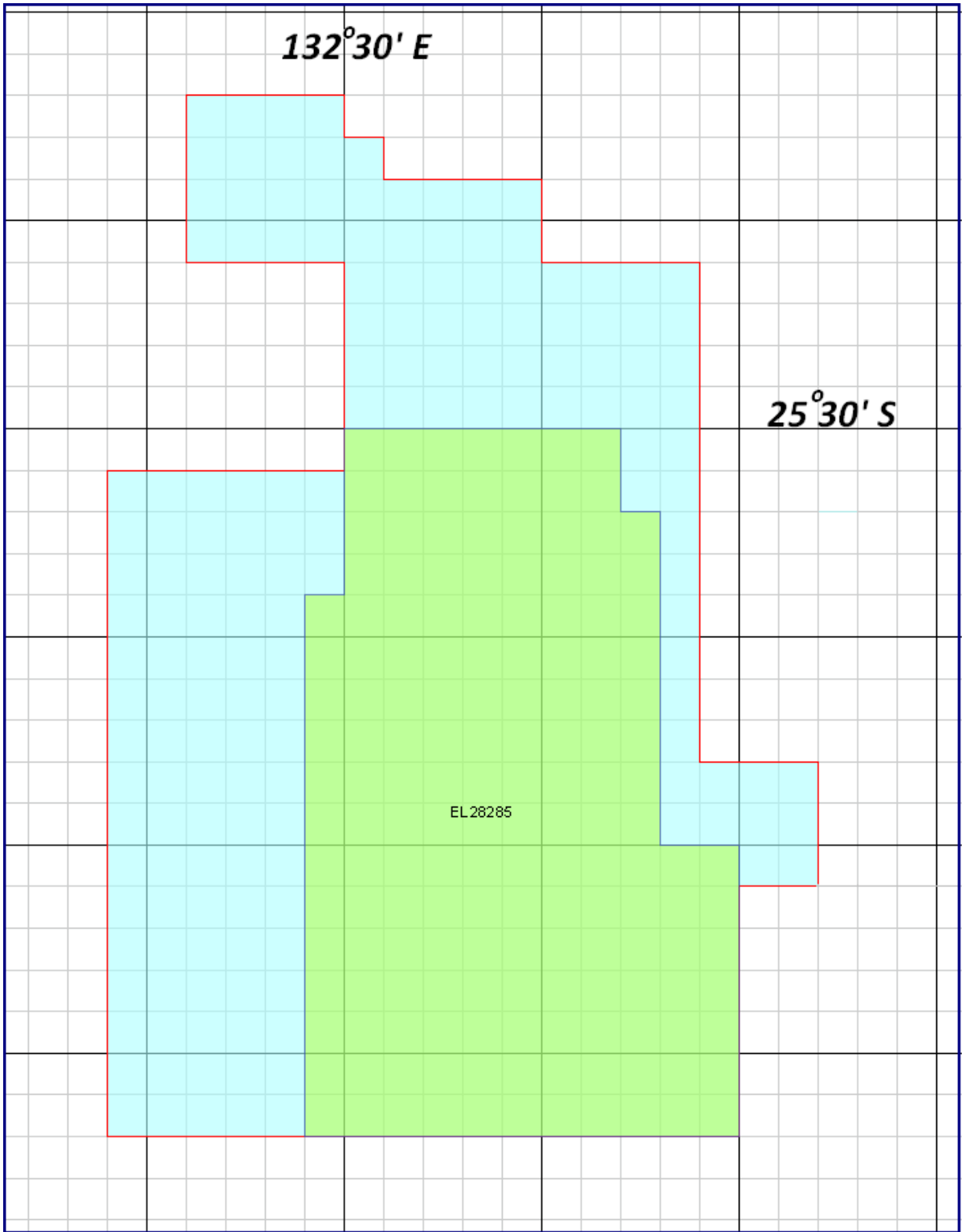
Figure 2: EL 28285 showing the relinquished 166 Blocks (blue)
