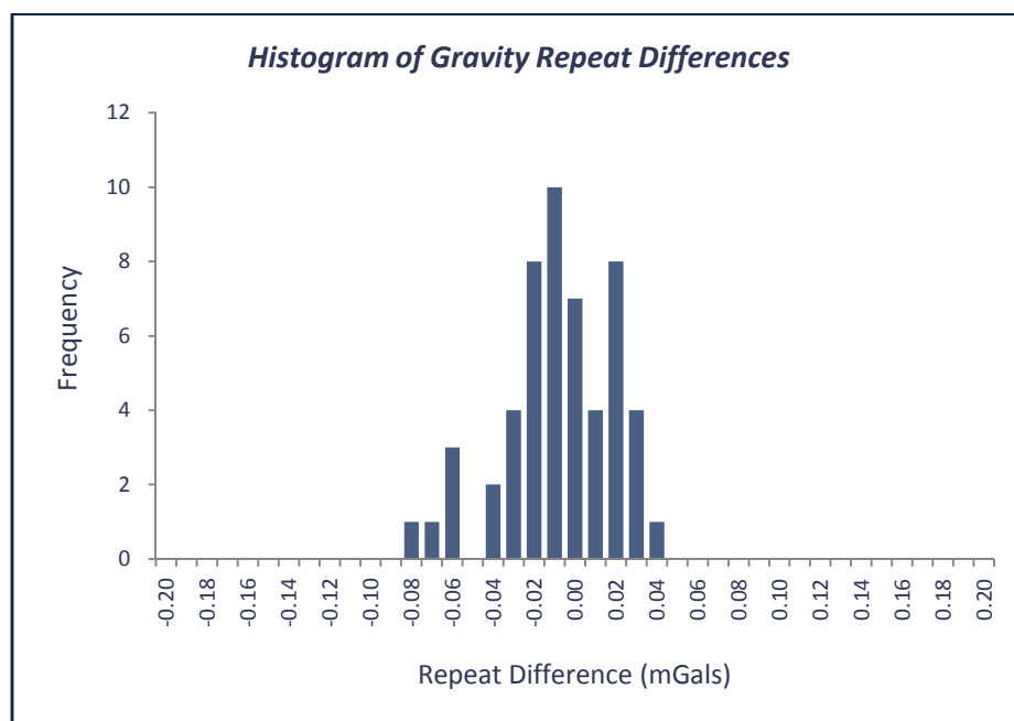
Figure 13: Histogram of Gravity Repeat Differences
