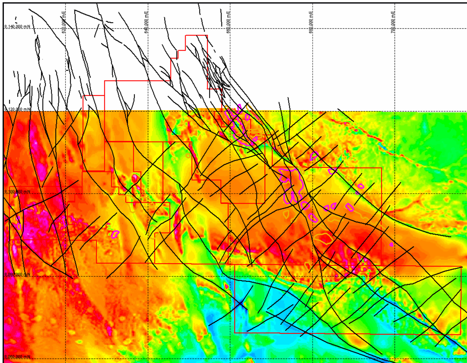
Figure 4. Radiometric anomalies shown on an image of the airborne magnetics data. Tan is uranium; magenta is potassium.
