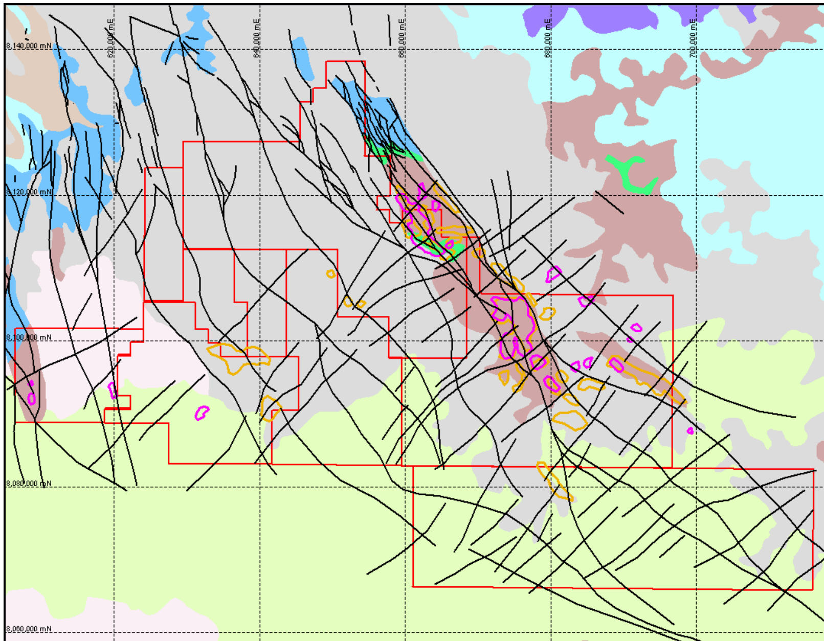
Figure 3. Radiometric anomalies on the NTGS geological interpretation. Tan is uranium; magenta is potassium.
