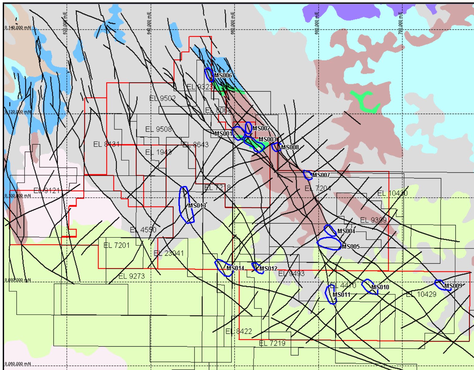
Figure 1. NTGS geological interpretation map showing distribution of targets in relation to main architectural elements discerned during the interpretation. Uranium targets in blue; base metals targets in red. See target description tables for details and ranking.
