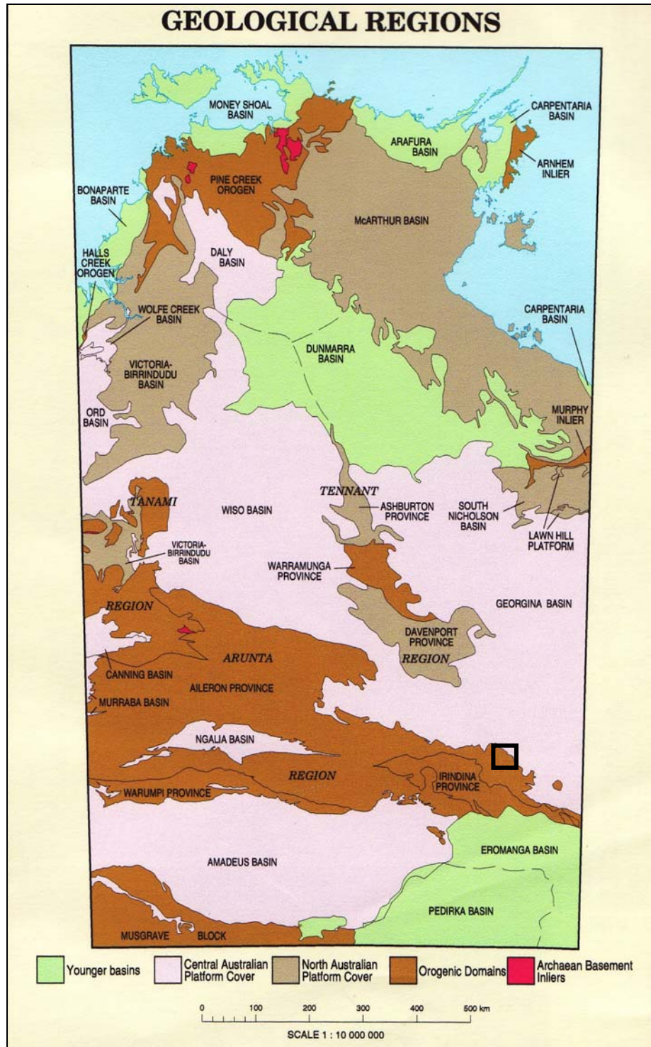
Figure 2. Geological Regions of the Northern Territory (image from Ahmad and Scrimgeour, 2004) showing the approximate area of interest for Jervois project area and EL 26318.
