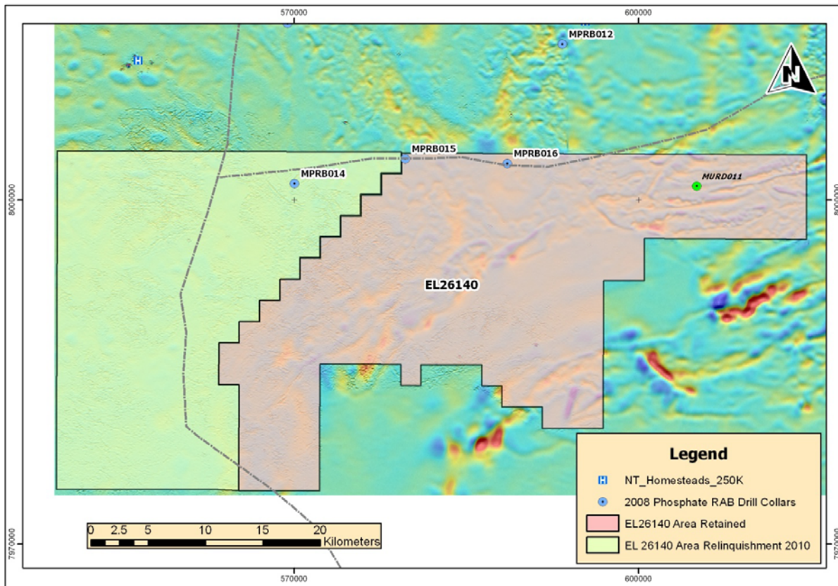
Figure 6: Location of RAB drill hole on EL 26139, with colour TMI magnetics image
