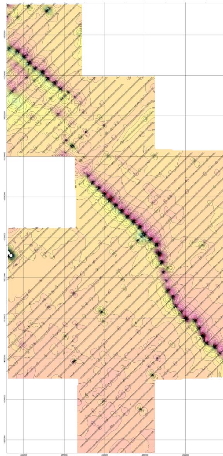
Figure 4 \Delta T map of Geomagnetism of EL25311
