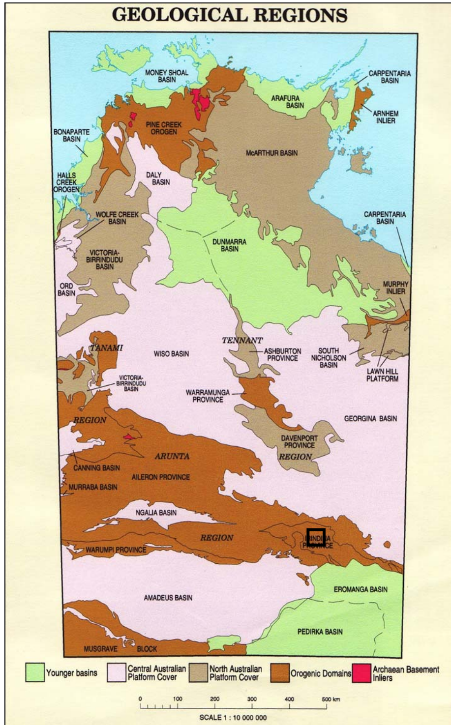
Figure 2. Geological Regions of the Northern Territory (image from Ahmad and Scrimgeour, 2004) showing the approximate area of interest for Hammer Hill project area and EL 26520.
