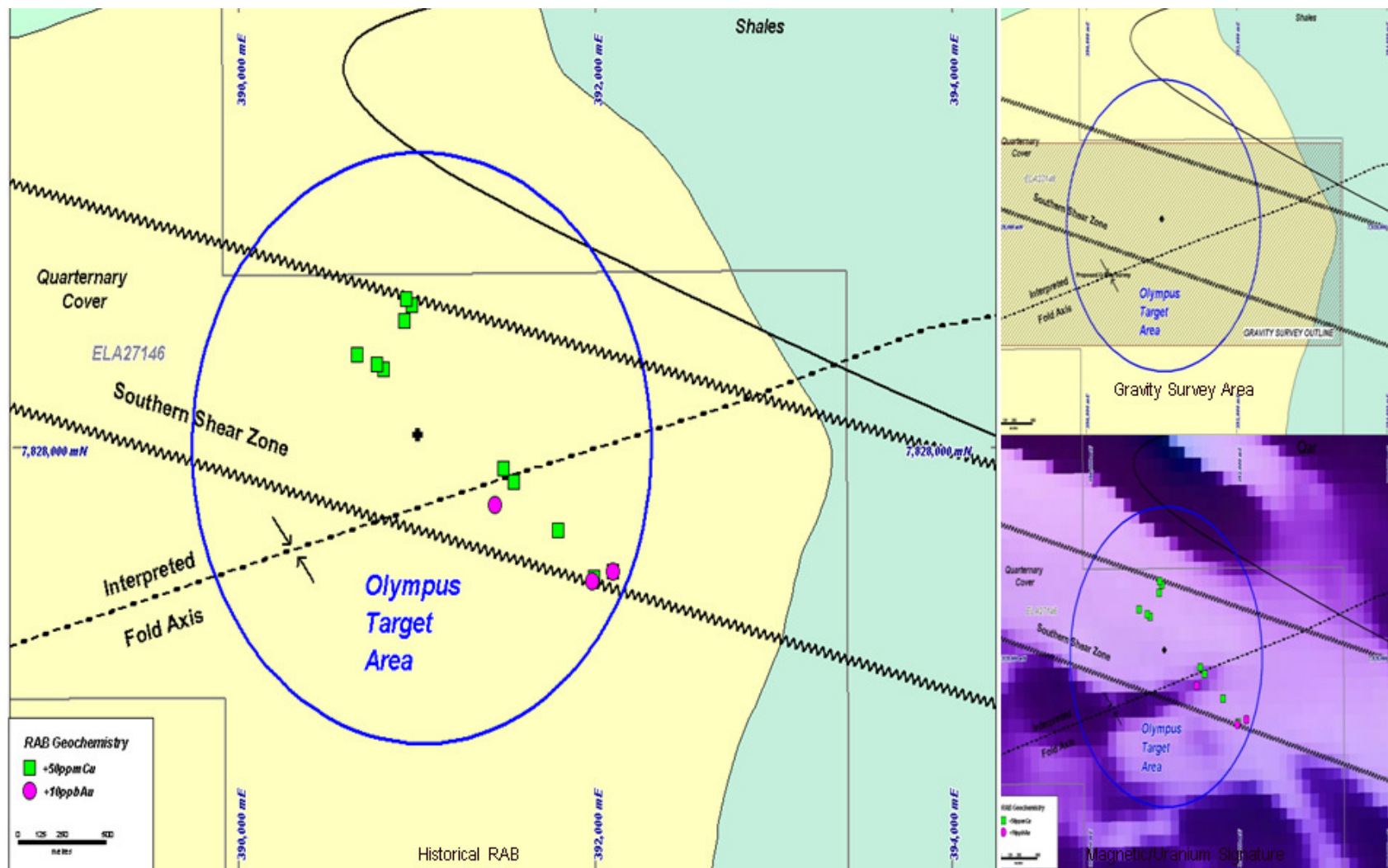
Figure 8 EL27145 Geological Interpretation
