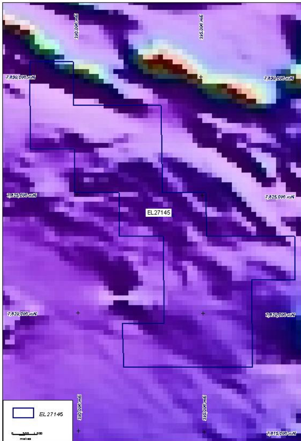
Figure 6 EL27145 Regional TMI Image (From NTGS Strike Database)
