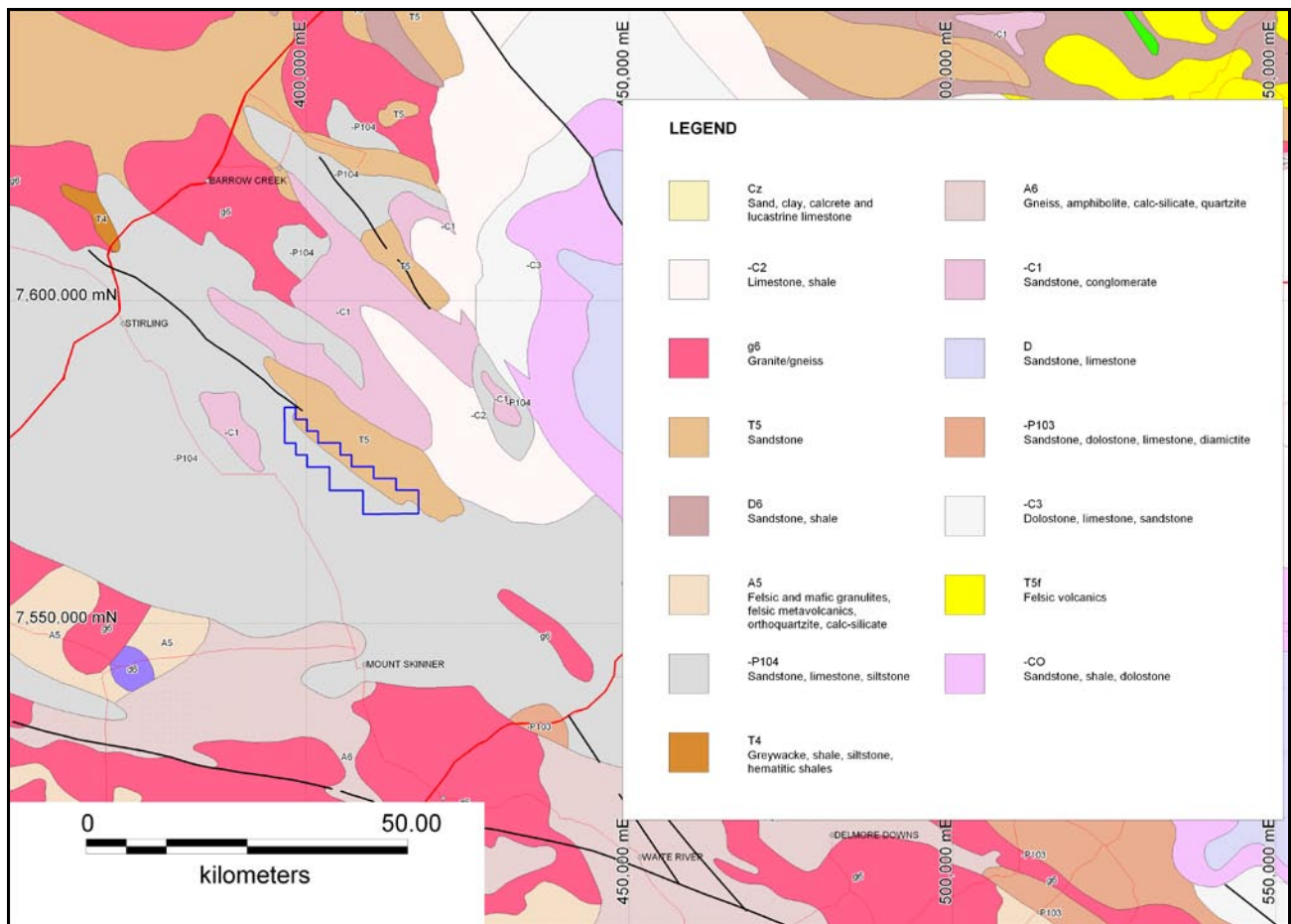
Figure 3. Simplified Geology of Project Area (compilation of various published maps)
