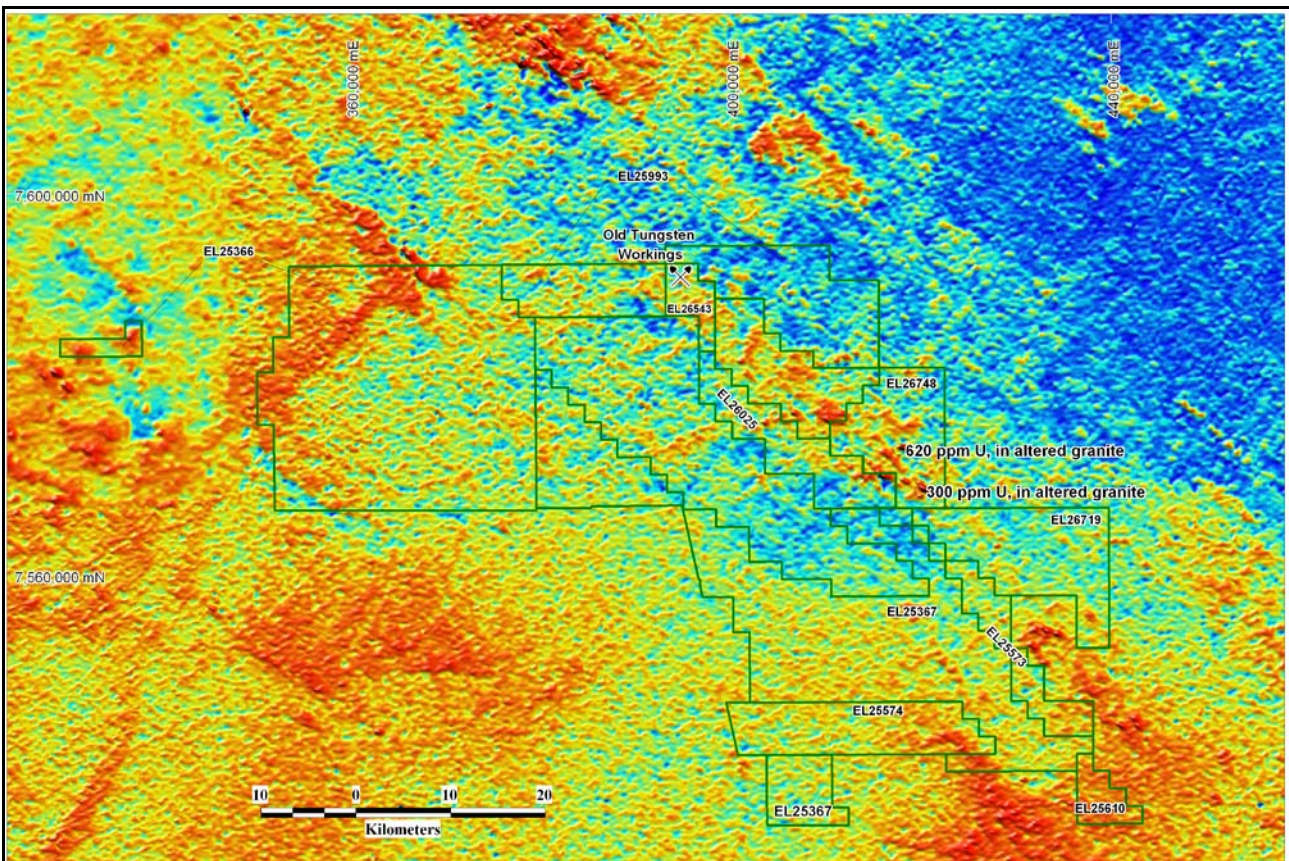
Figure 7. Regional (400m line spaced) Uranium radiometric image
