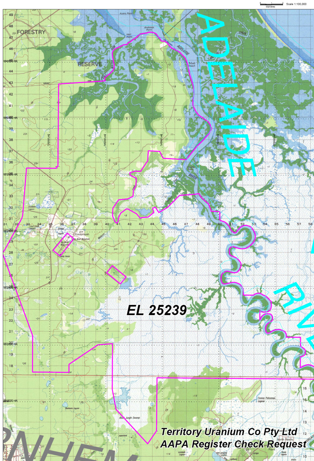
Figure 1: EL25239 Tenement Location
