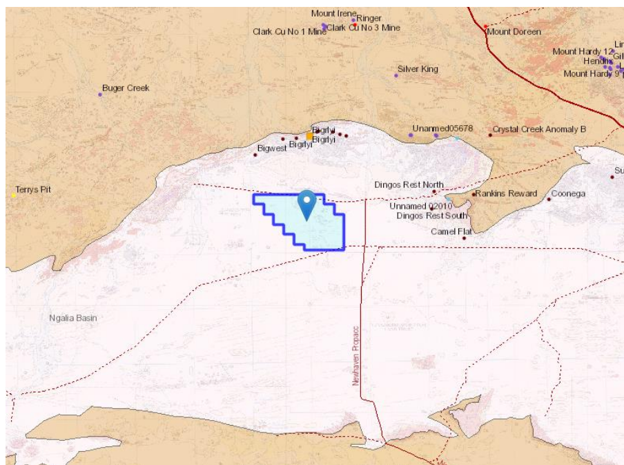
Figure 3: Regional Geology
