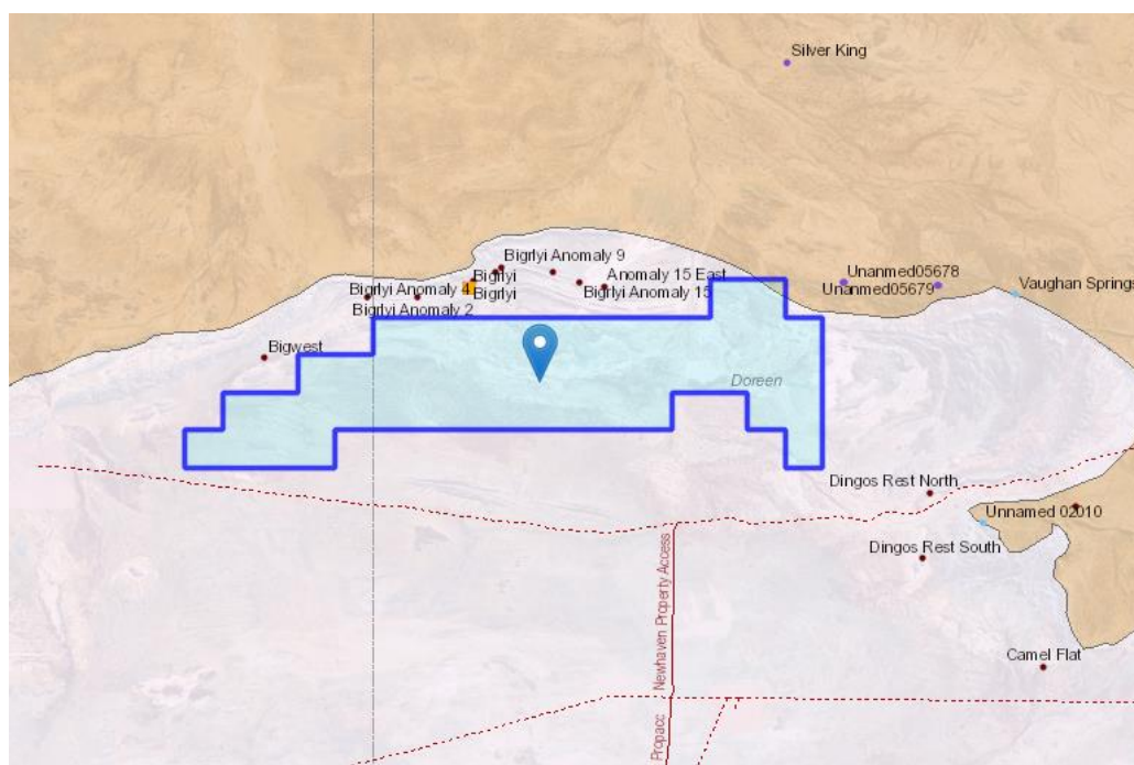
Figure 3: Regional Geology
