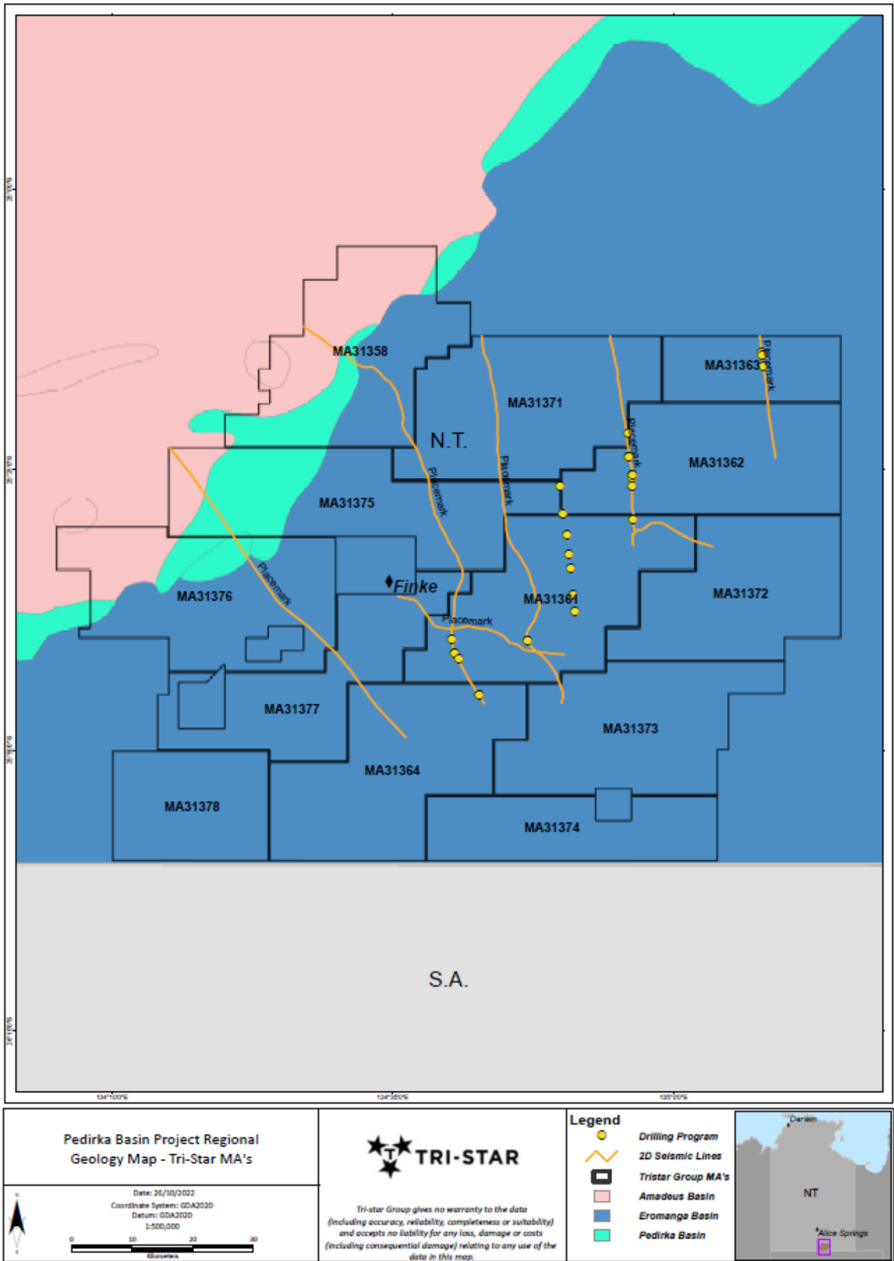
Figure 6. Historical Seismic and Drill Site Map
