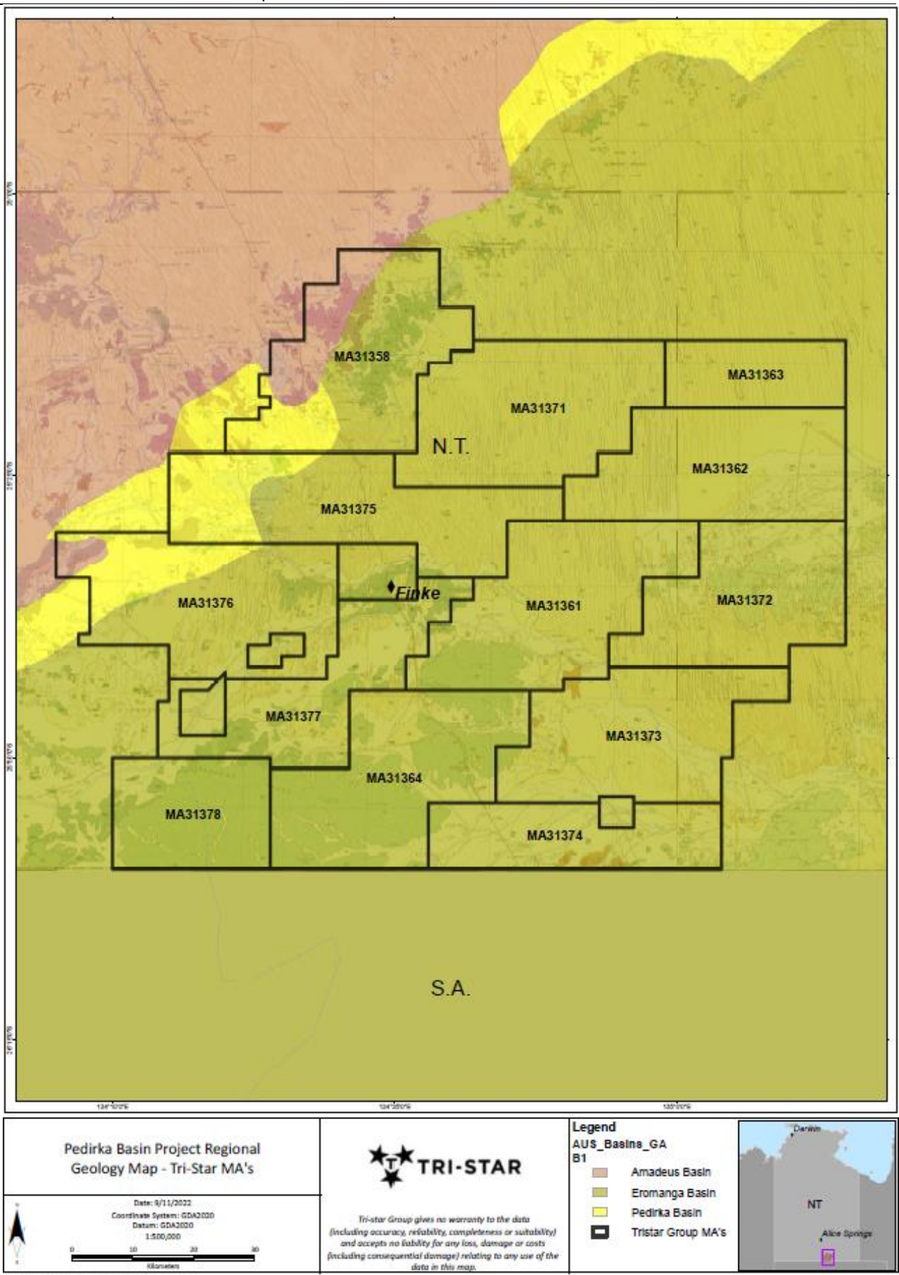
Figure 3. Pedirka Basin Project – Regional Geology
