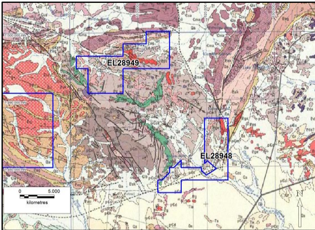
Figure 3: Published geology of the tenement area.
