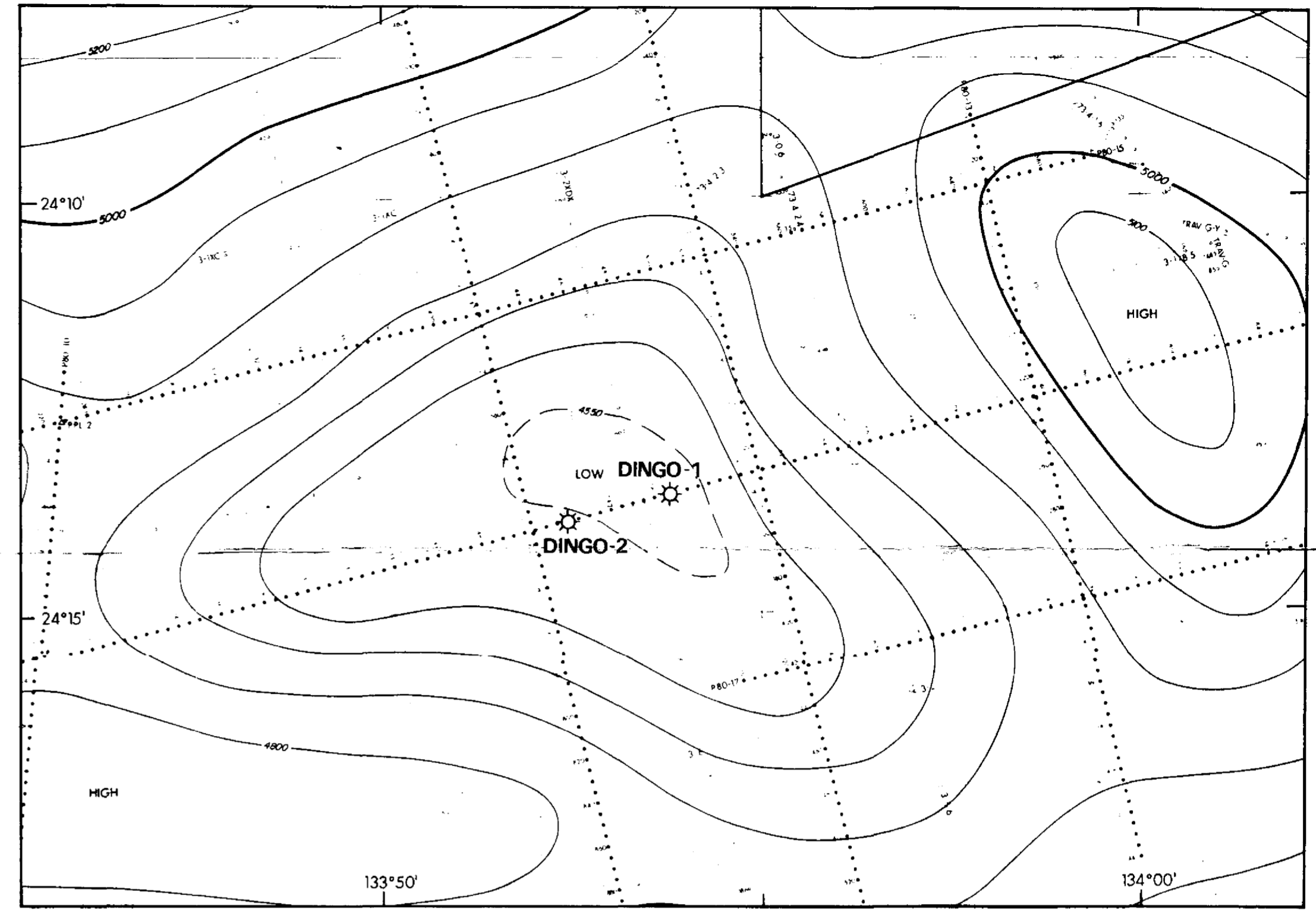
Average Velocity Contours Near Top of First Gas Pay Contour Interval: 100 m/sec
