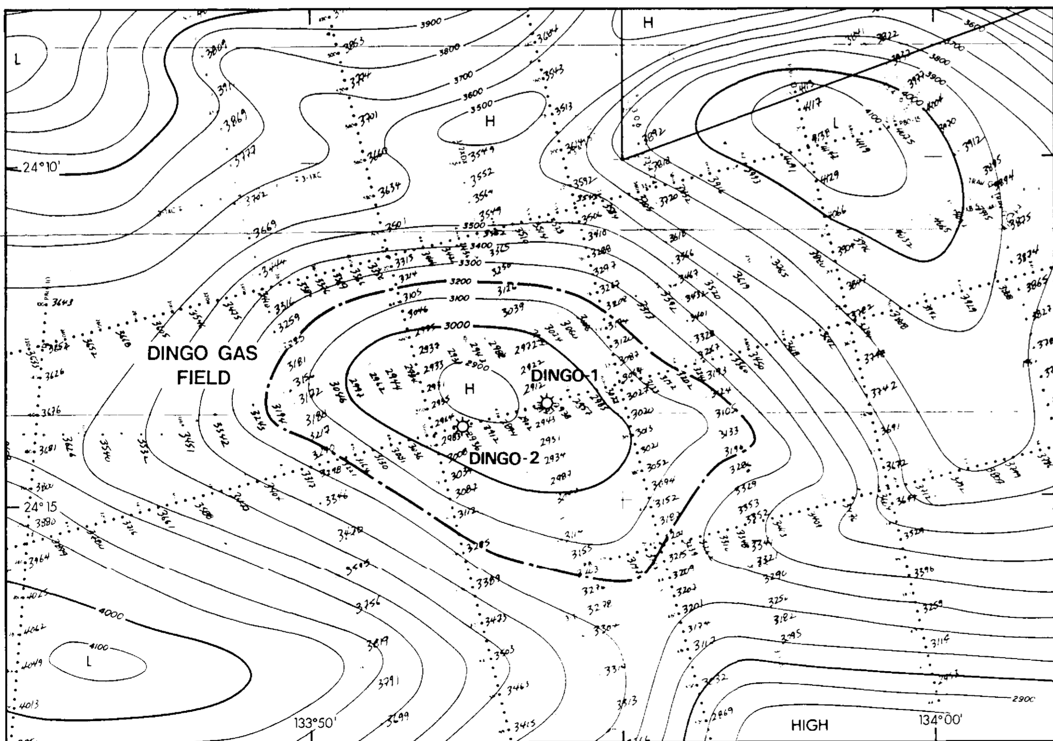
Depth Contours Near Top of First Gas Pay Contour Interval: 100m
