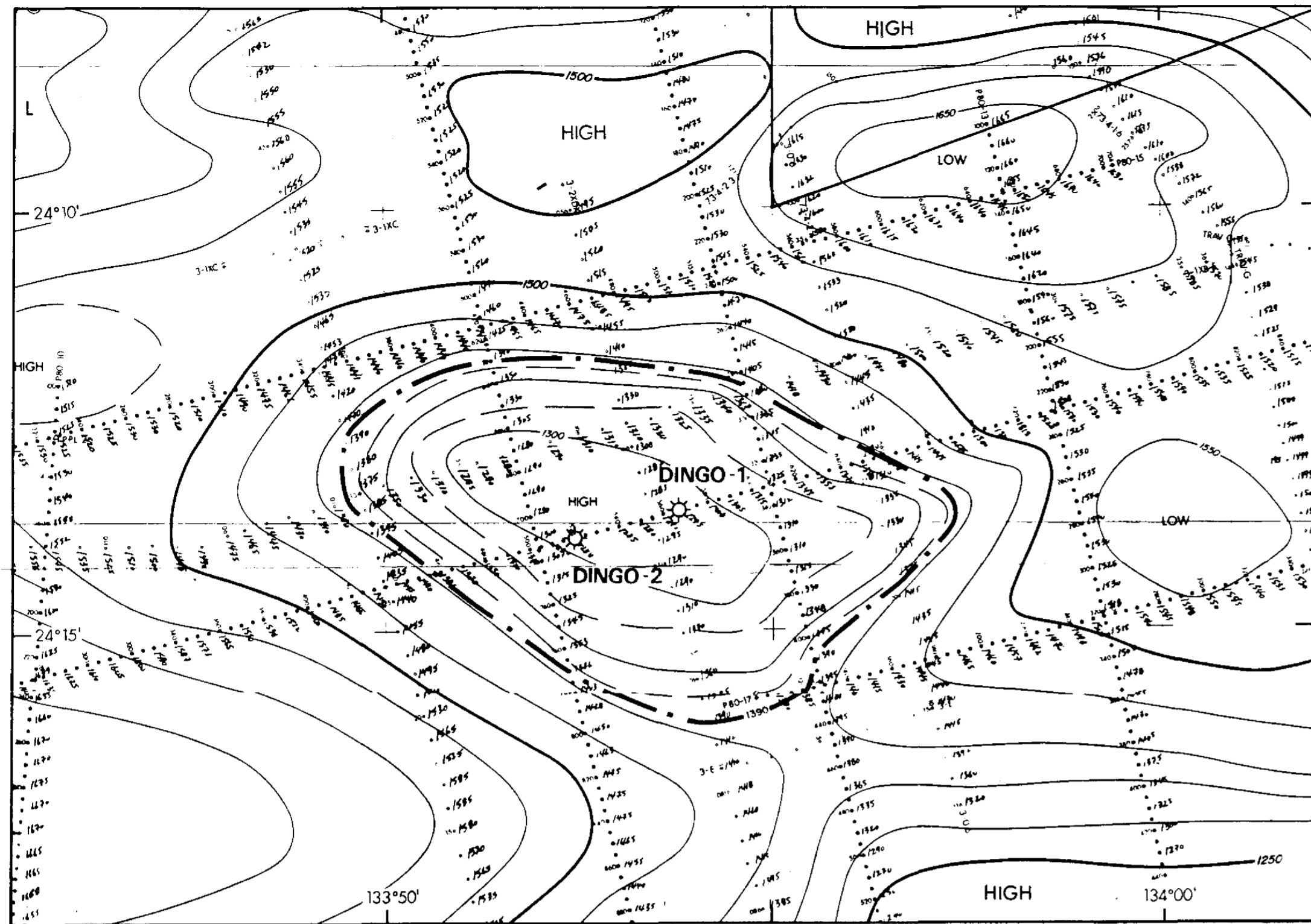
Two Way Time Contours Near Top of First Gas Pay Contour Interval: 50 msec
